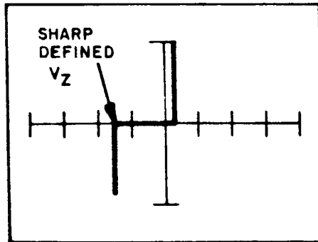
Figure 3-24. Signature of a Good Zener Diode in the Medium 1 Range at 60Hz
