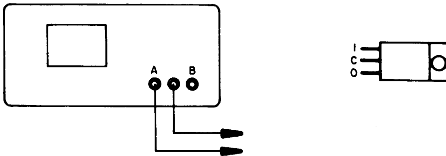
Figure 7-12. Test Connections to a 7805 +5V Regulator
