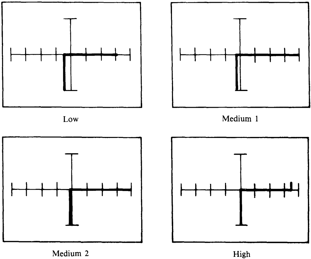
Figure 4-30. G-D Signatures of an N-Channel JFET (2N5638) at 60Hz
