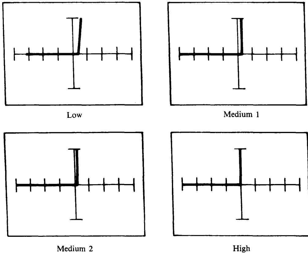
Figure 3-6. Signatures of a Silicon Diode at 60Hz
