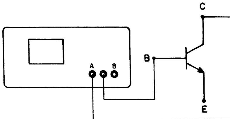
Figure 4-8. Collector-Base Test Connections
