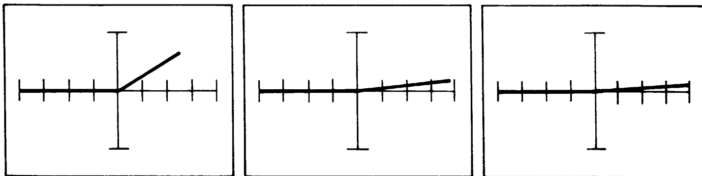
100K Resistor
