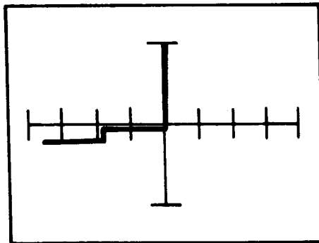
figure 8-39. Signature variations of a H11C3 as a function of pulse level for the maximum pulse width, at 60Hz.
