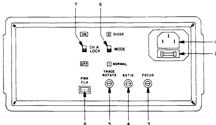
Figure 2-2. Back Panel
