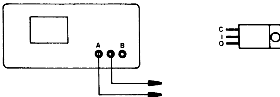
Figure 7-18. Test Connections to the 7905
