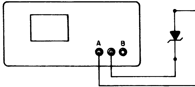
Figure 3-22. Zener Diode Test Connections
