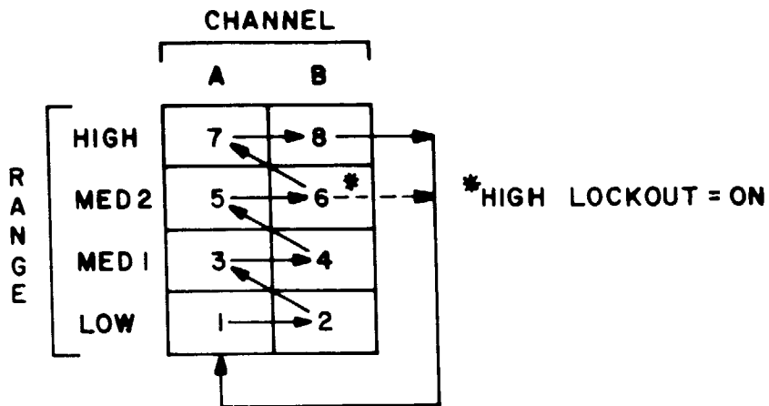
Figure 2-5. Auto/Alternate Sequence
