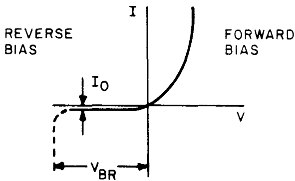
Figure 3-4. The Volt-Ampere Characteristic of a Semiconductor
