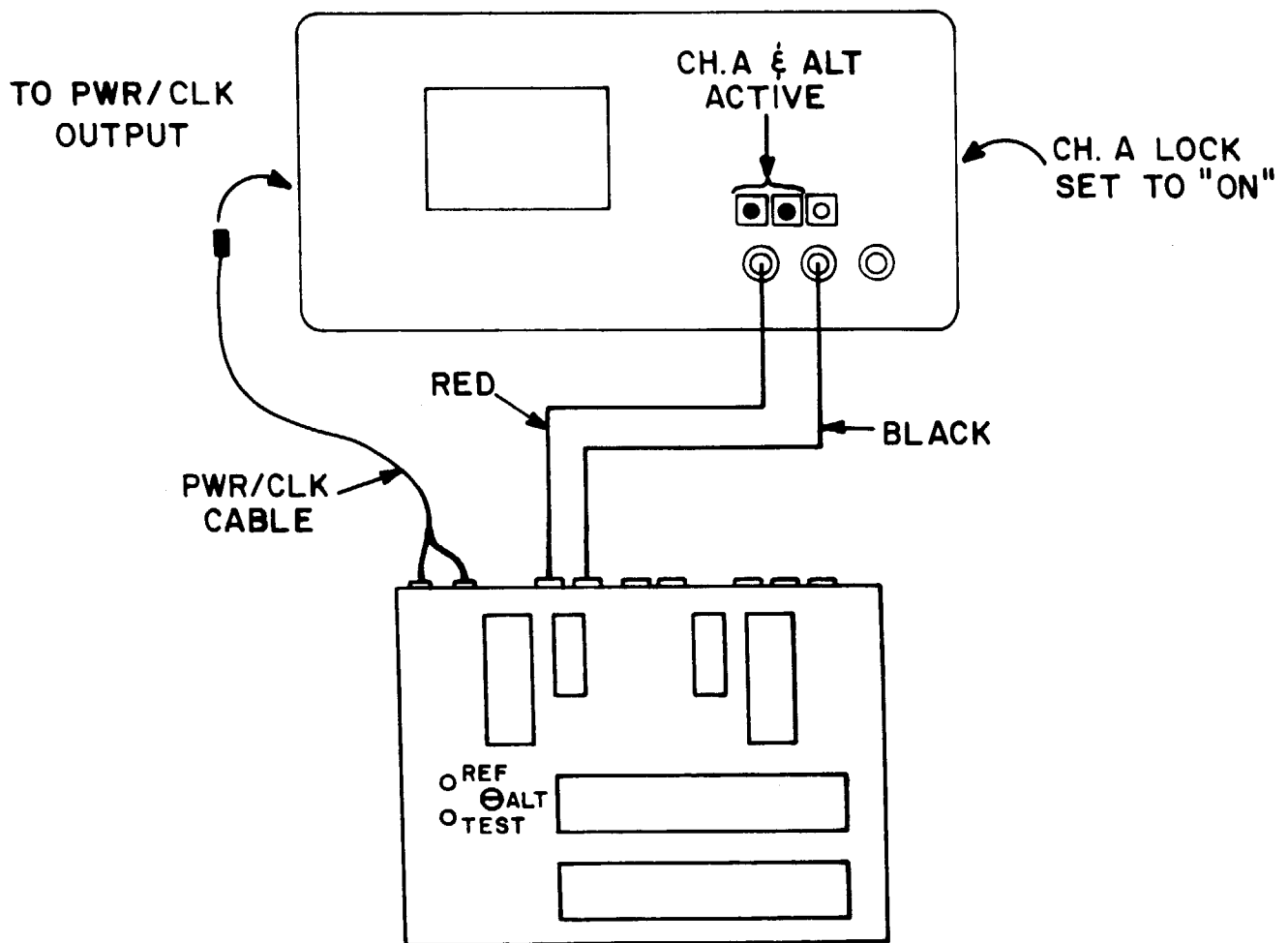
Figure 2-7. Tracker/Switcher Interconnection
