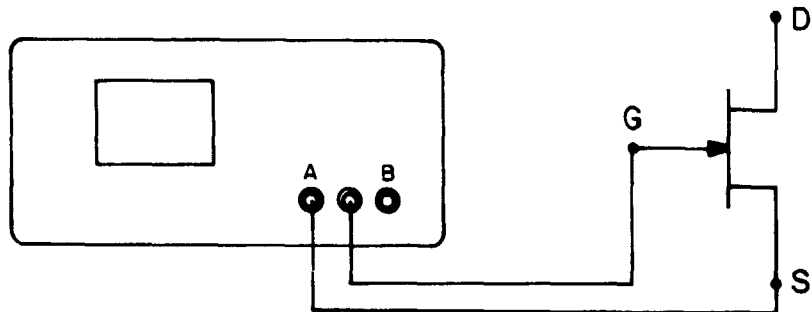
Figure 4-31. Source-Gate Test Circuit
