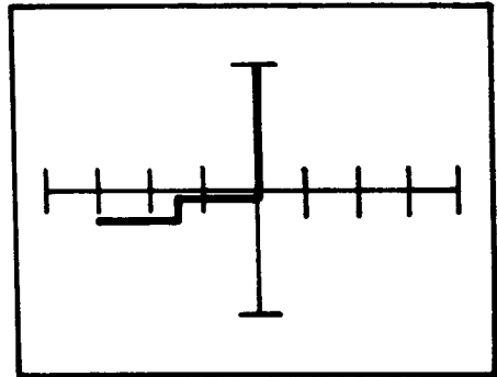
figure 8-39. Signature variations of a H11C3 as a function of pulse level for the maximum pulse width, at 60Hz.
