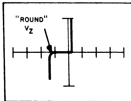
Figure 3-25. Signature of an Inferior Zener Diode in the Medium 1 Range at 60Hz
