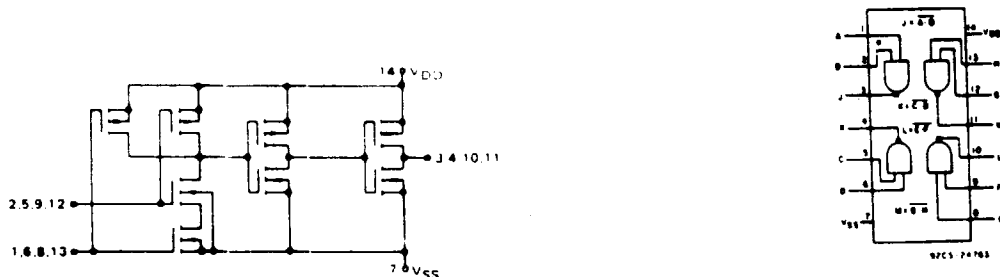
Figure 7-47. Schematic and Connection Diagram of a MC14011B
