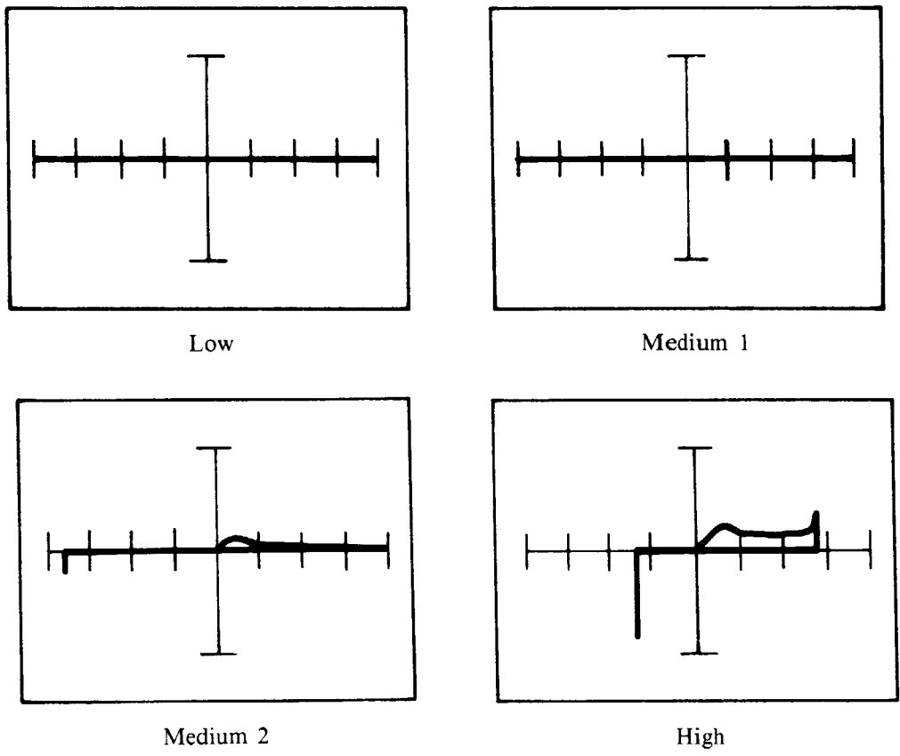
Figure 4-40. G-D Signatures of an N-channel Enhancement Mode MOSFET (VN10KM) at 60Hz
