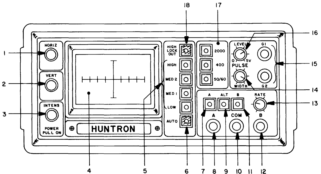
Figure 2-1. Front Panel
