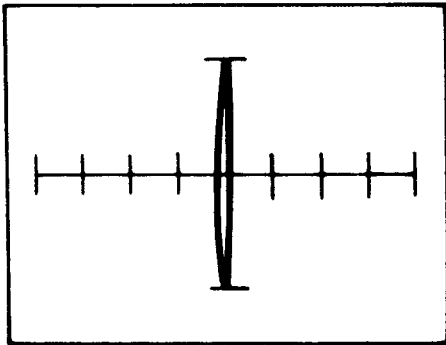
High, 1uF, 60Hz
