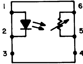
Figure 8-45. Pin Configurations of a CLM-51 Photocell Optocoupler.
