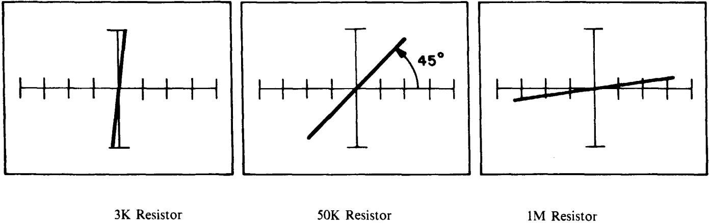
Figure 5-4. Effects of Resistance on Rotation Angle — High Range
