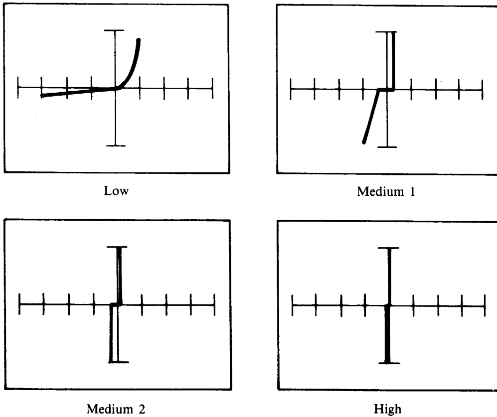
Figure 7-38. Signatures Between the V_{cc} Pin and Ground Pin of a 7410 at 60Hz.
