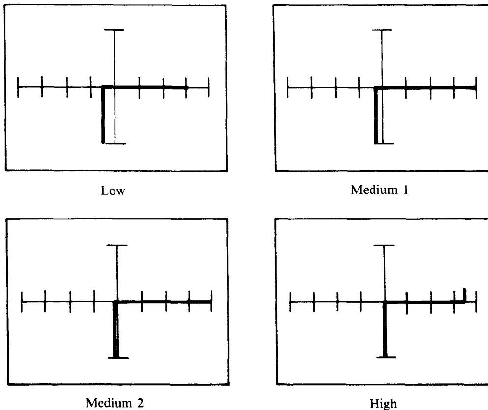
Figure 4-32. S-G Signatures of an N-Channel JFET (2N5638) at 60Hz
