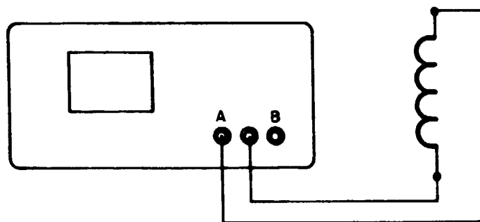
Figure 5-7. Inductor Test Connections
