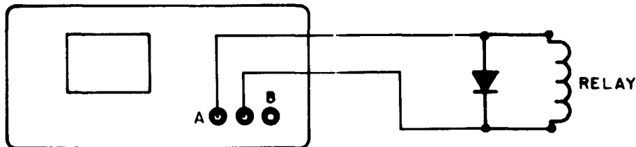
Figure 6-17. Inductance/Diode Combination
