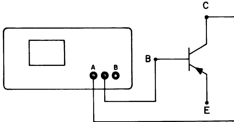
Figure 4-15. Collector-Base Test Connections
