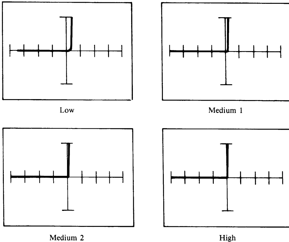
Figure 7-25. Signatures Between Pin 2 and Pin 1 of an LM555 Timer at 60Hz
