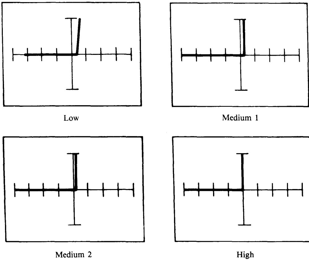
Figure 1-6. Signatures of a Silicon Diode at 60Hz
