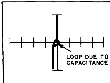
Figure 3-27c. Signature of a PN2222 B-E Junction in High Range at 2KHz
