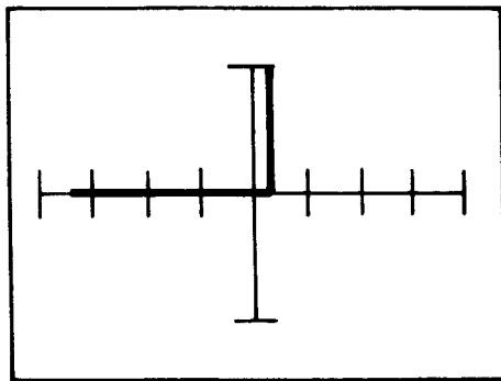
Low Test Signal is not high enough to cause Zener Breakdown
