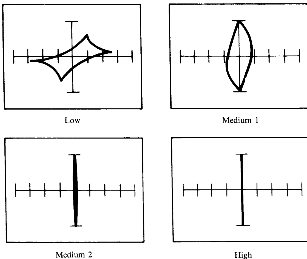
Figure 5-9. Signatures of 490mH Ferrite Inductor Tested at 60Hz
