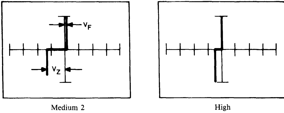
Figure 3-27b. Signatures of a PN2222 B-E Junction in the Medium 2 and High Ranges at 60Hz
