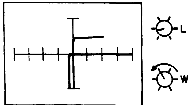
Effect of the Width Control at Constant level Medium 1 Range, at 60Hz
