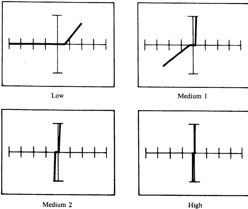
Figure 7-41. Signatures Between the V_{cc} Pin and Ground Pin of a 74LS32 at 60Hz
