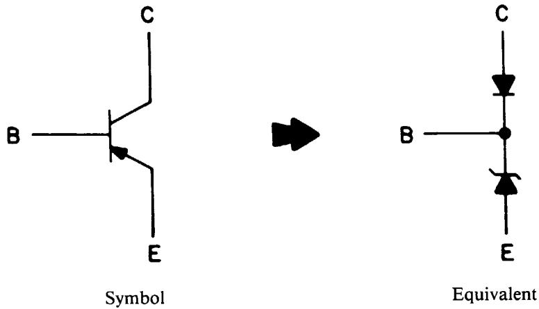
Figure 4-10. PNP Transistor
