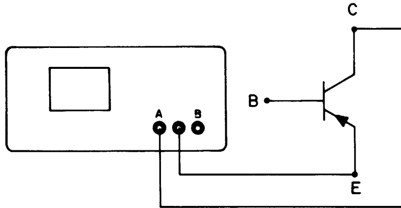
Figure 4-13. Collector-Emitter Test Connections
