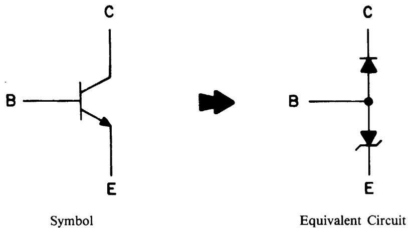
Figure 4-3. NPN Transistor
