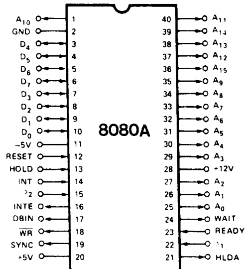
Figure 7-83. Pin Configuration of an 8080A
