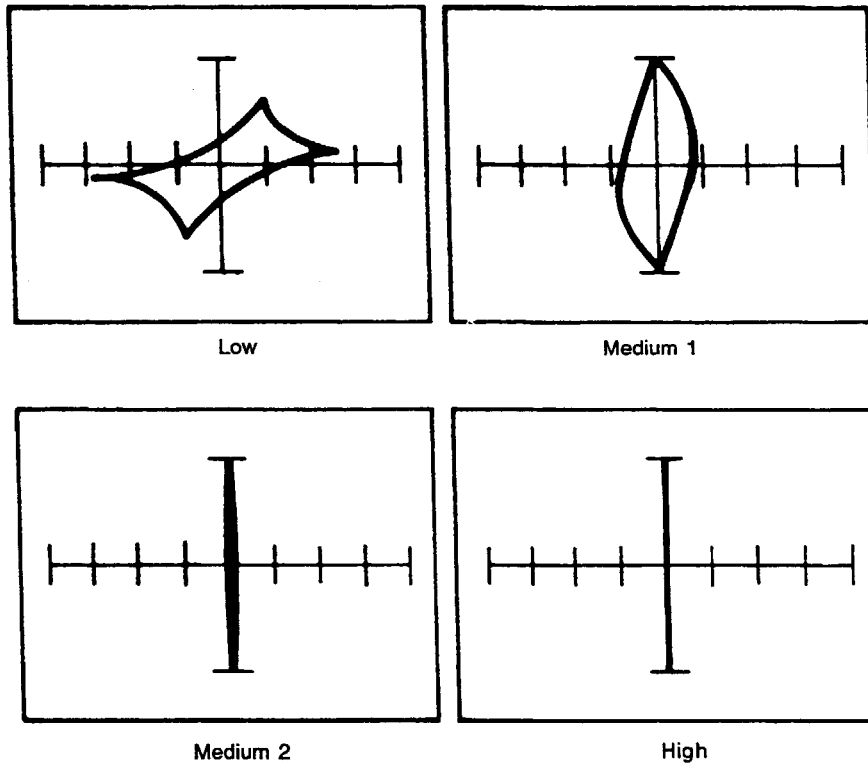
Figure 7-7. Signatures of a 490mH Ferrite Inductor Tested at 60 Hz.
