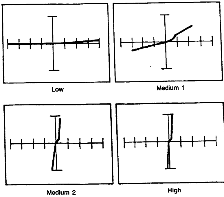
Figure 12-25. Signatures Between Pin 5 (Control Voltage) and Pin 1 of an LM555 Timer at 60 Hz.
