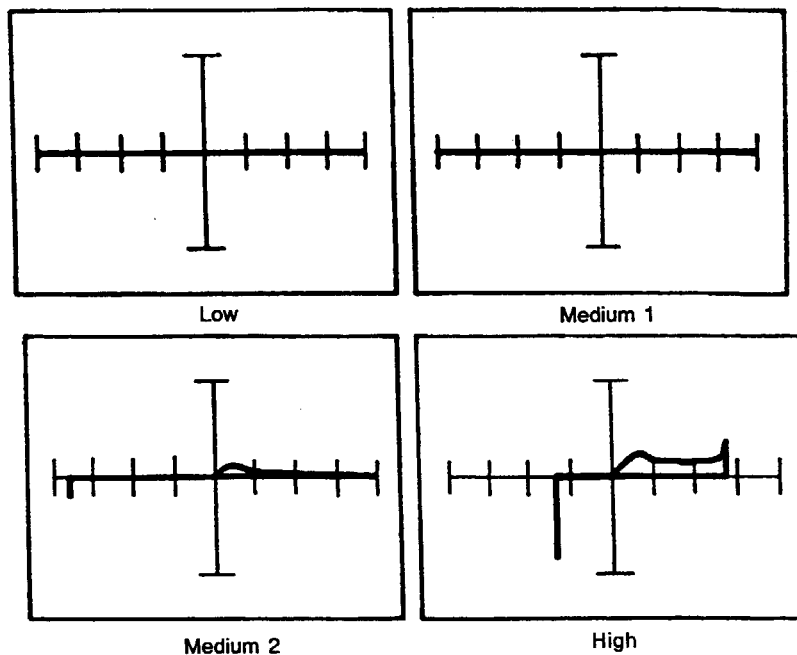
Figure 9-26. Signatures of an N-Channel Enhancement Mode MOSFET (VN10KM) at 60 Hz. Drain with Gate as Common.
