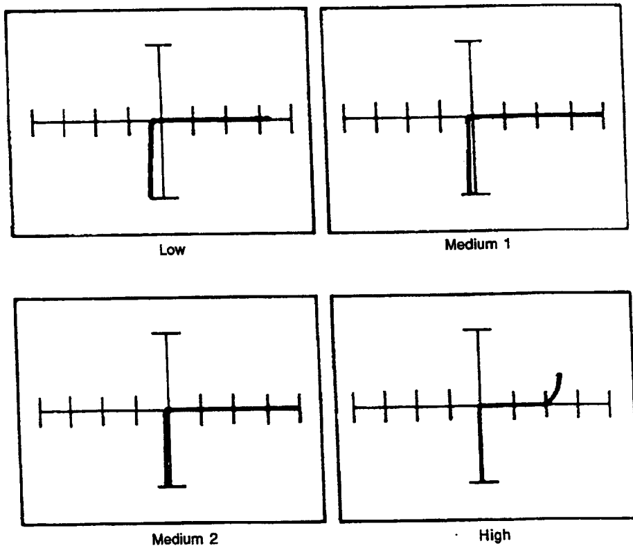
Figure 12-67. Signatures Between an Output Pin and the Ground Pin of a 6301-1J at 60 Hz.
