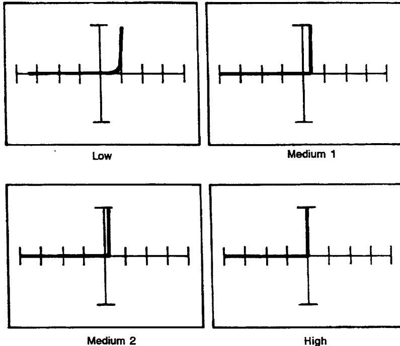
Figure 13-6. Signatures of a Good HV15F Diode.
