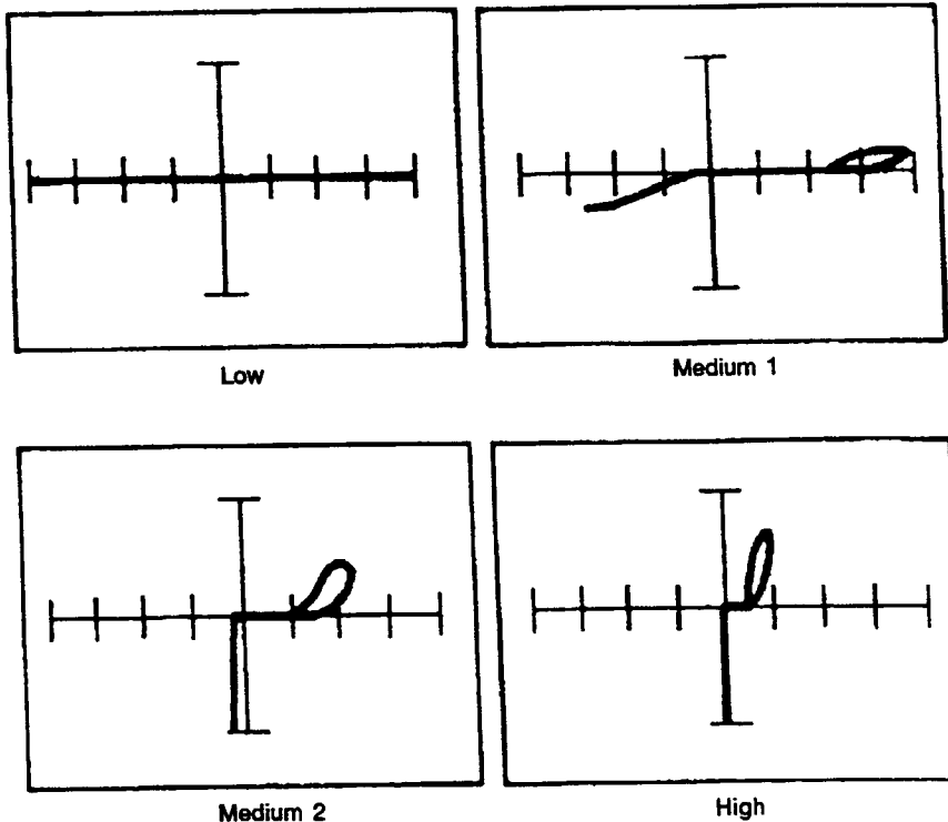
Figure 12-44. Signatures Between an Input Pin and V_{SS} - V_{DD} of a 4011B at 60 Hz.
