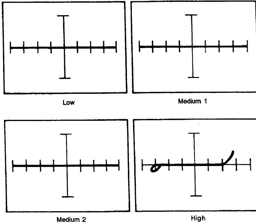
Figure 12-7. Signatures Between Pin 2 (Inverting Input) and Pin 4 (V-) of an LM1458 at 60 Hz.
