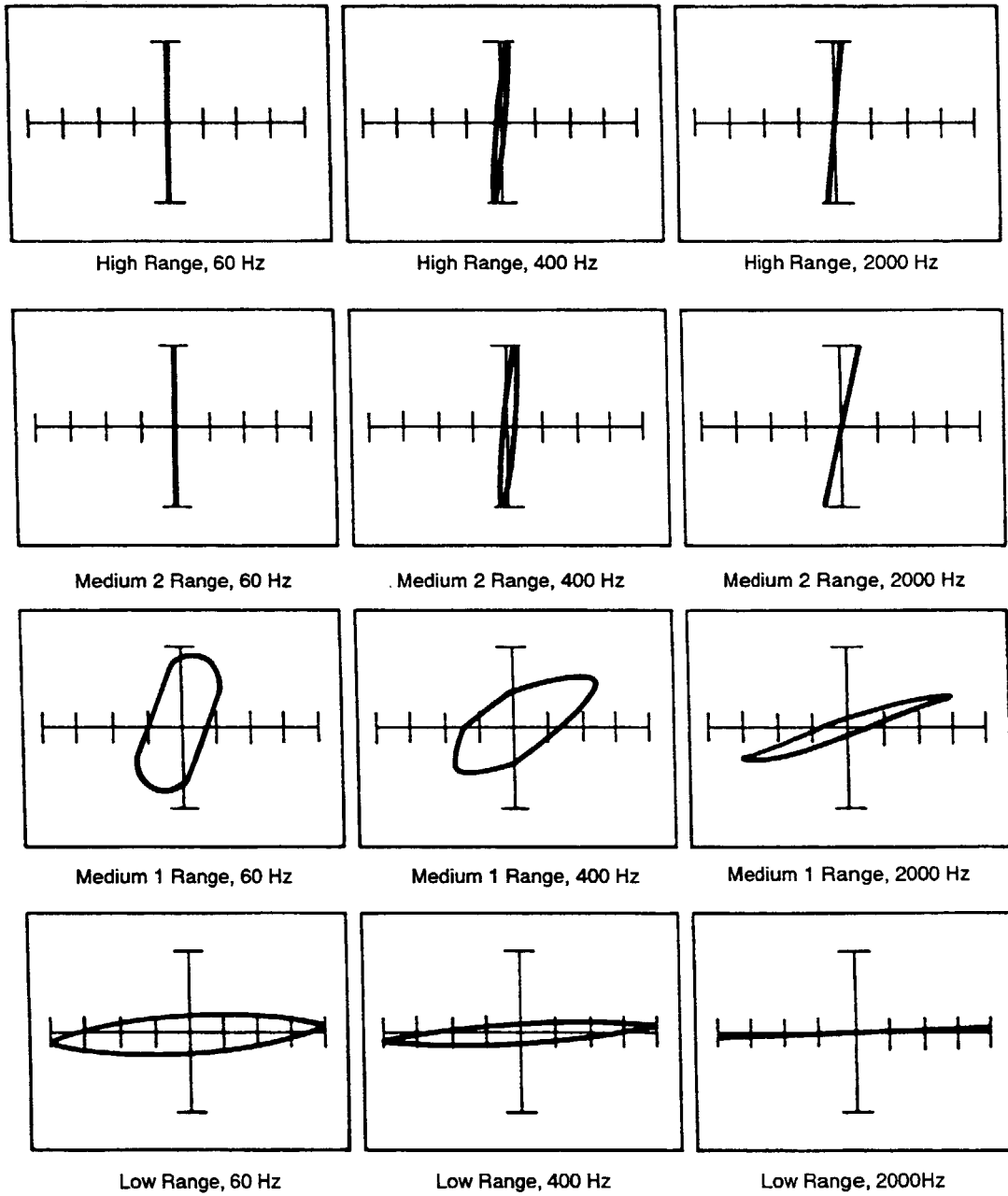
Figure 7-6. Signatures of a 250mH Inductor.
