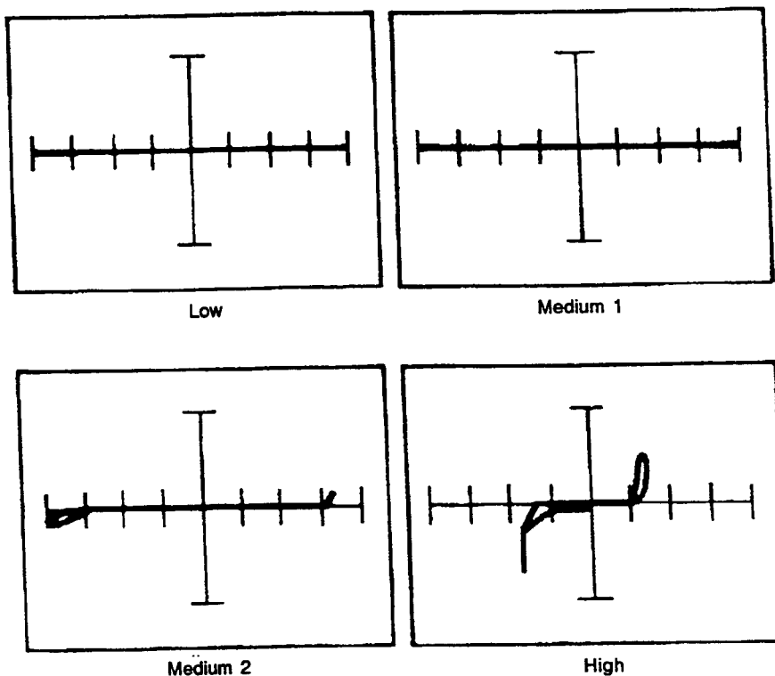
Figure 12-52. Signatures Between an Address Pin and the Ground Pin of a 2114A Static RAM at 60 Hz.
