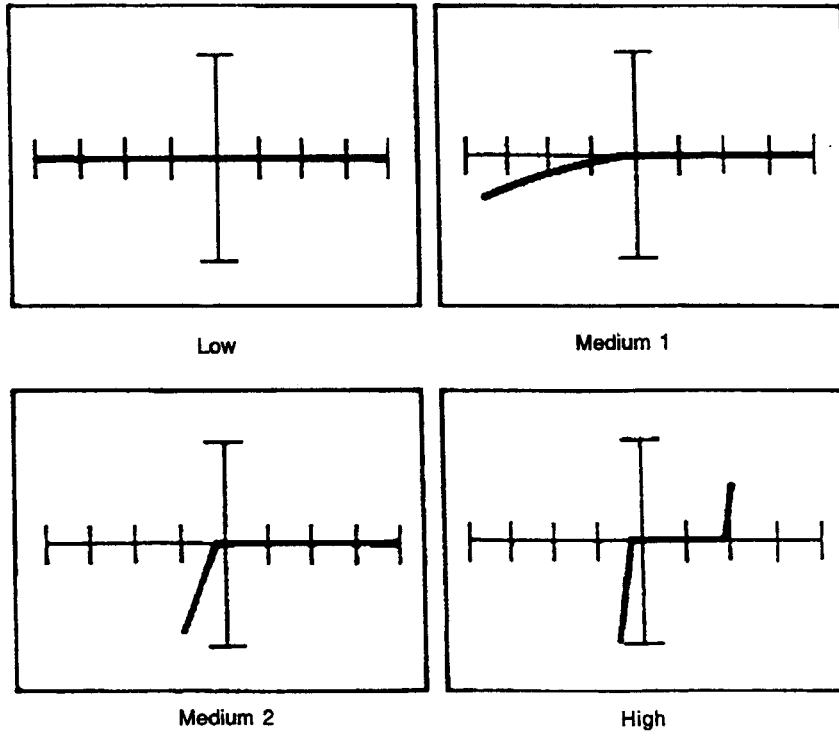
Figure 12-83. Signatures Between the +12V Pin and the -5V Pin of an 8080A at 60 Hz.
