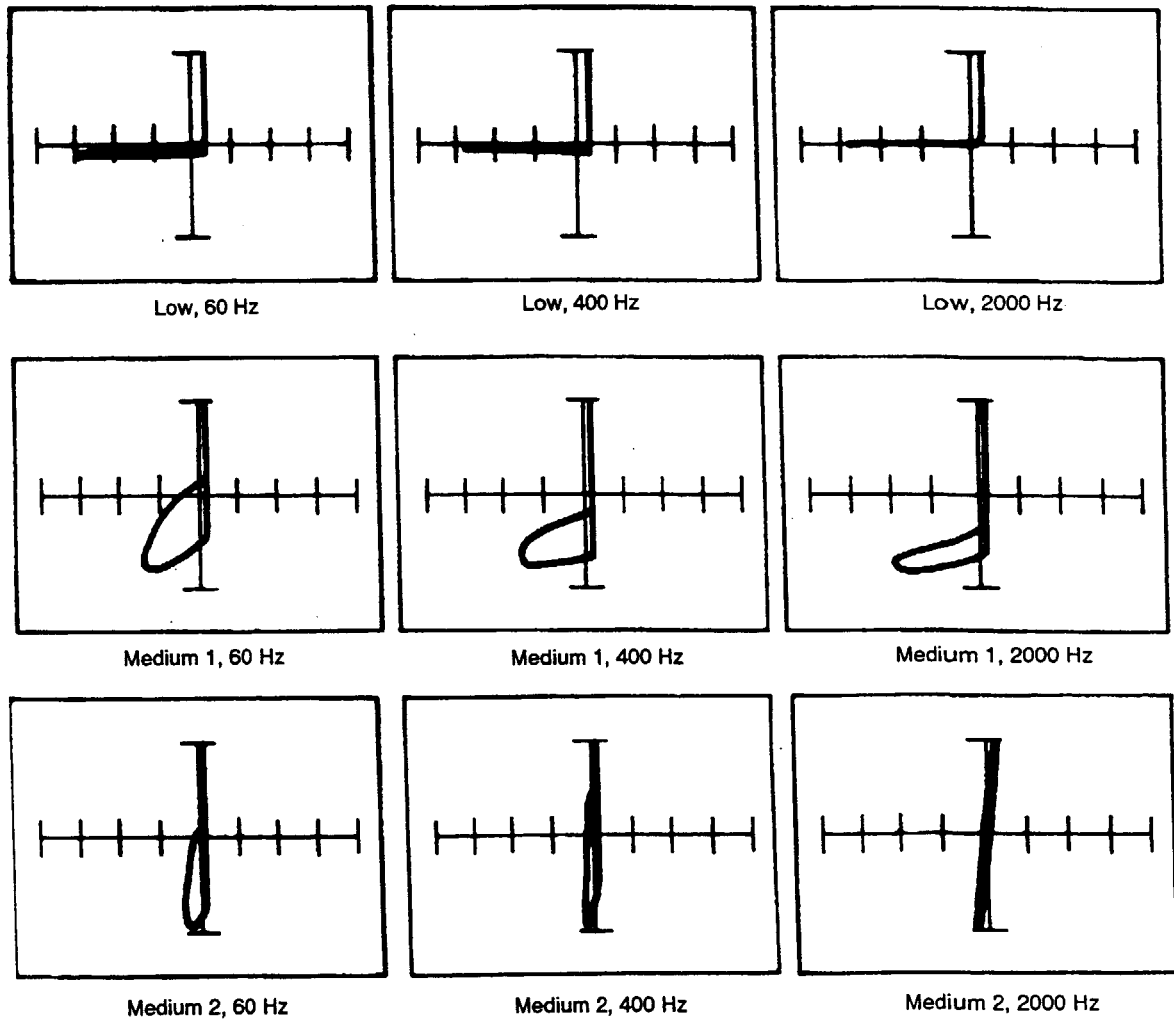
Figure 11-13. Signatures of a 1N4001 Diode in Parallel with an Aromat Relay HB1E-DC12.
