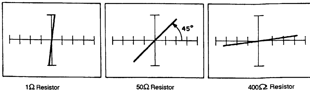
Figure 7-1. Effects of Resistance on the Rotation Angle - Low Range.
