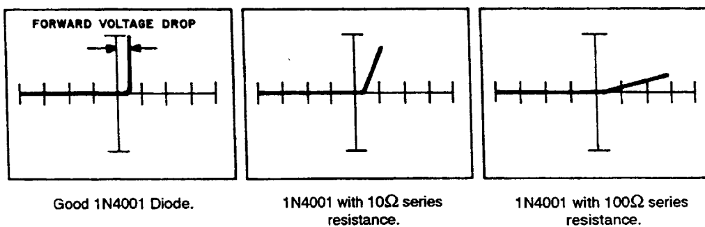
Figure 8-8a. Signature Deviation from a Good Diode in Low Range at 60Hz.
