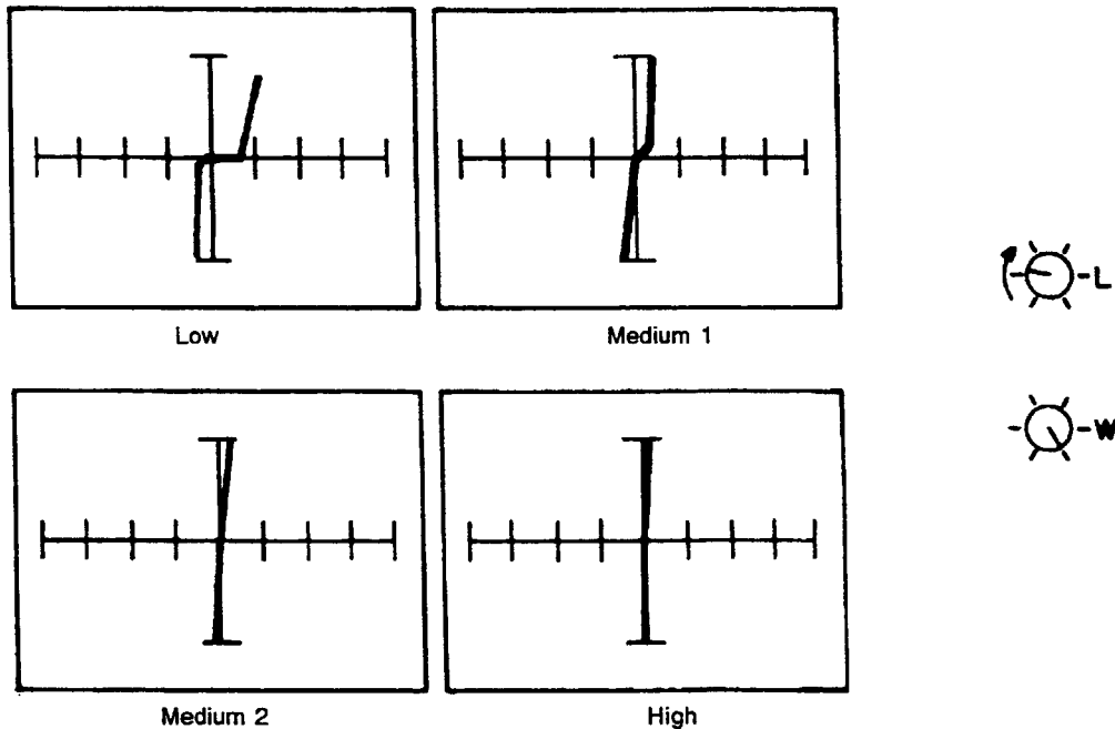
Figure 10-12. MT1-MT2 Signatures of a 2N6070 Triac with Gate Connected to the Pulse Generator at 60 Hz.
