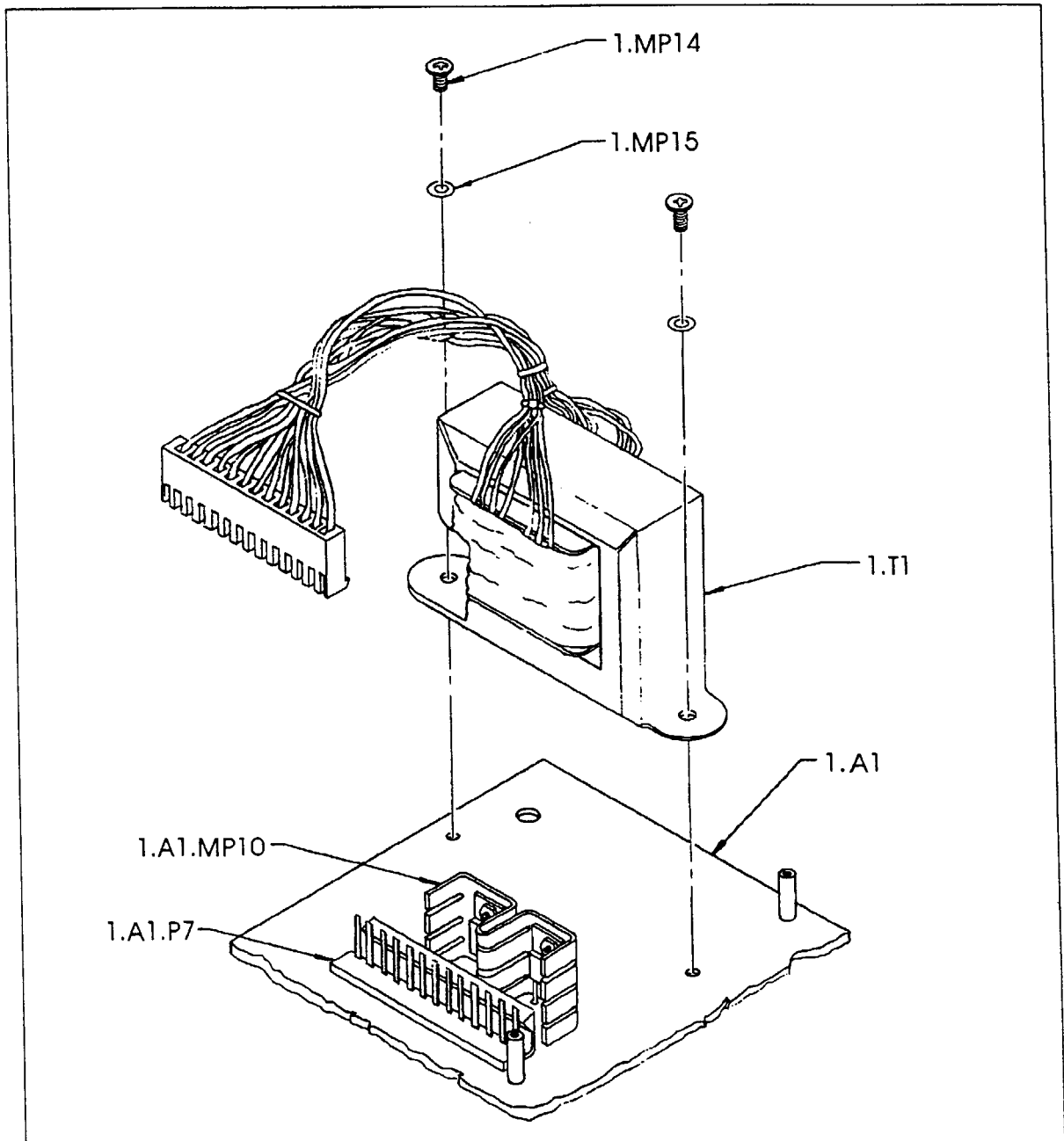
Figure 4-4. Power Transformer Removal.
