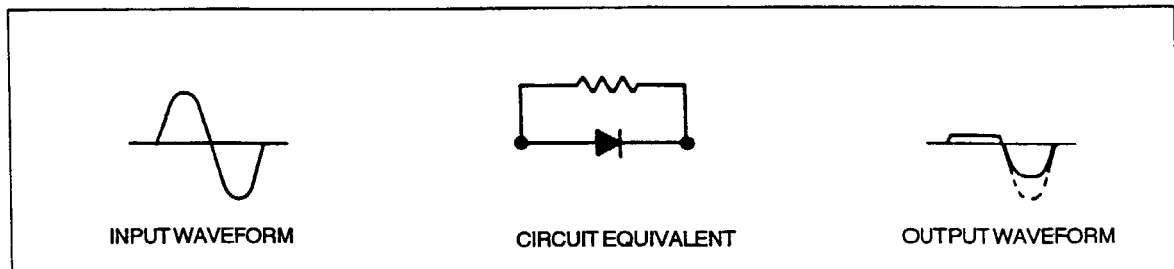
Figure 8-9a. Model of Diode with Leakage Resistance.
