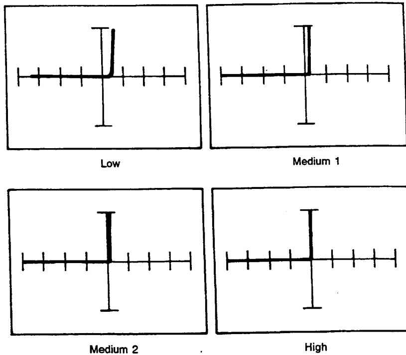
Figure 10-17. Signatures of the LED of a 4N25 at 60 Hz. Pin 1 with Pin 2 as Common.
