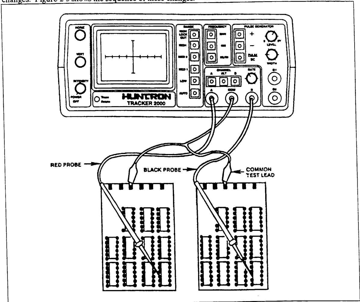
Figure 2-4. Alternate Mode Setup.
