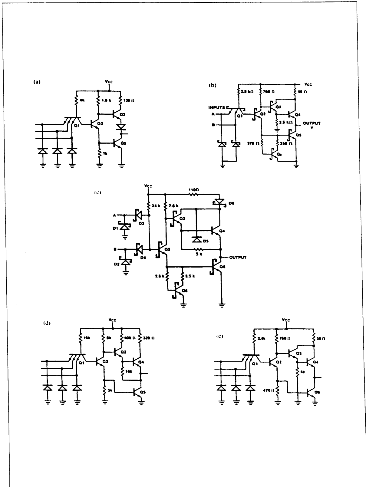
Figure 12-31. Various TTL Implementations.
