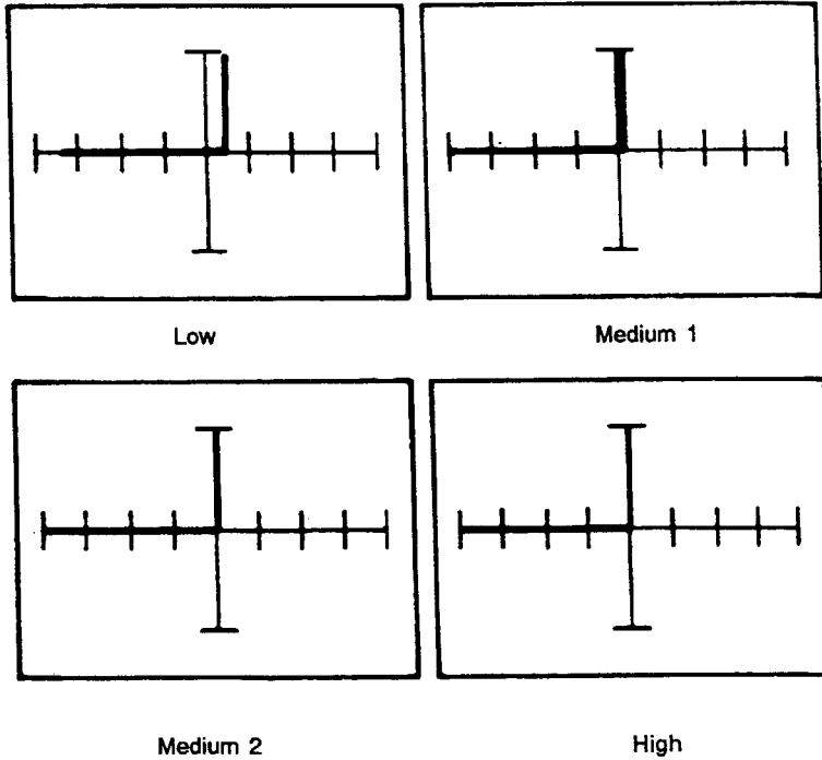
Figure 10-36. Signatures of the LED part of a MOC3010 at 60 Hz. Pin 1 with Pin 2 as Common.
