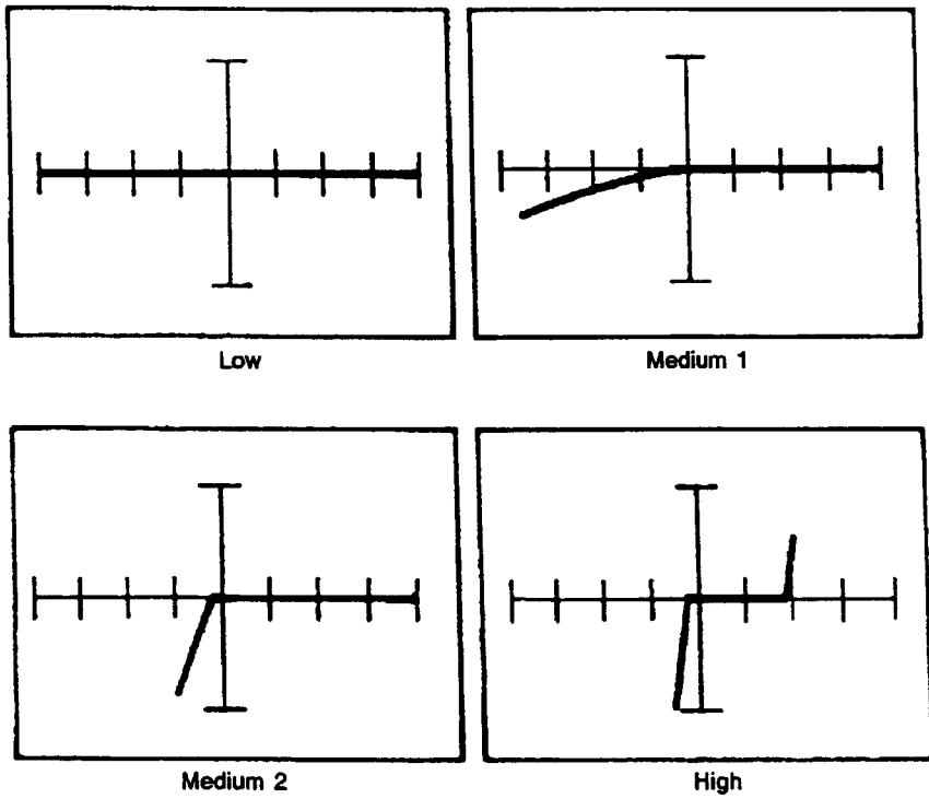
Figure 12-82. Signatures Between the +5V Pin and the -5V Pin of an 8080A at 60 Hz.
