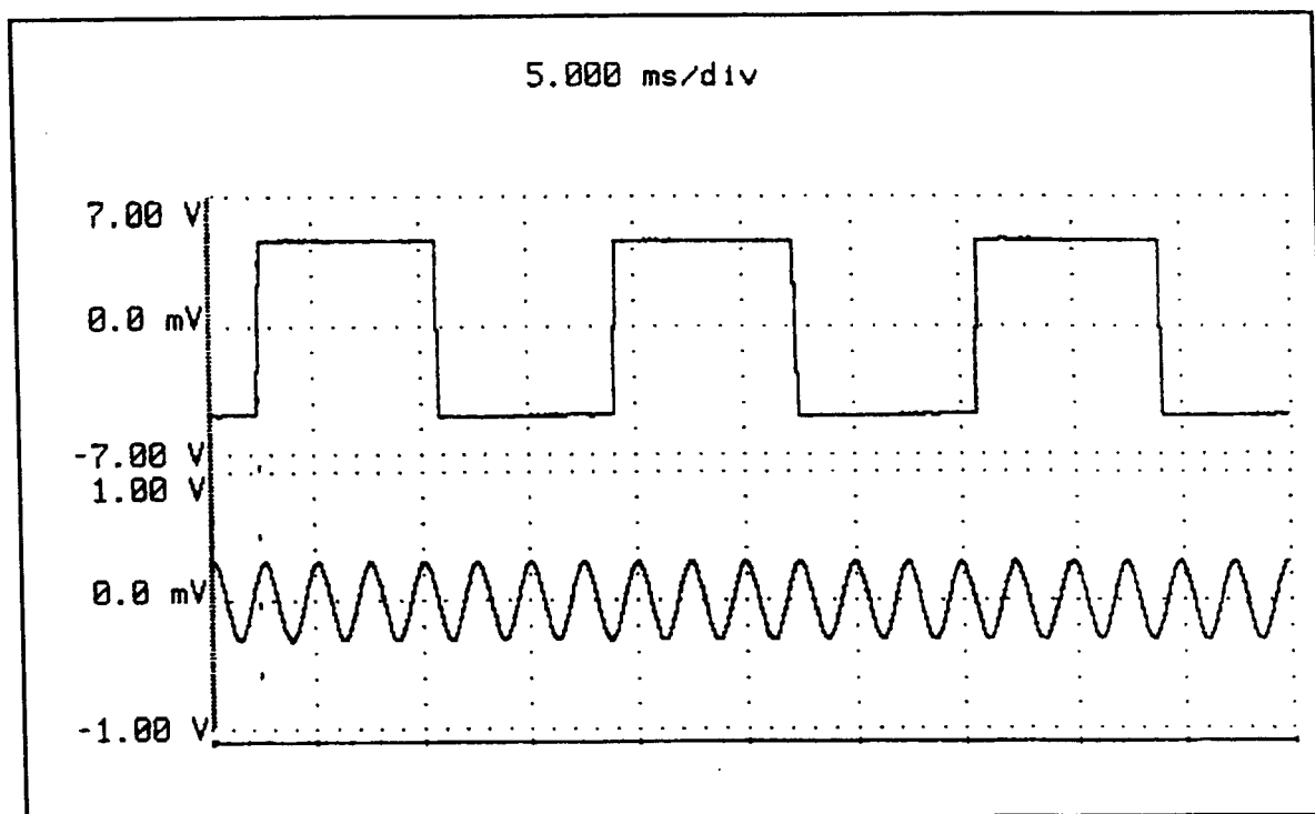
Figure 4-17. Signal PCB Waveforms: TP1 & TP9 - Settings: 400 Hz.
