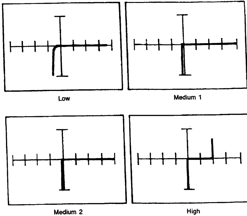
Figure 12-41. Signatures Between the Enable Pin and the Ground Pin of a 74LS125 at 60 Hz.
