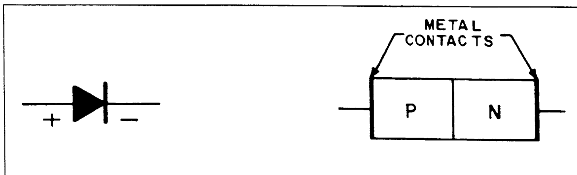
Figure 8-1. Diode Symbol.
