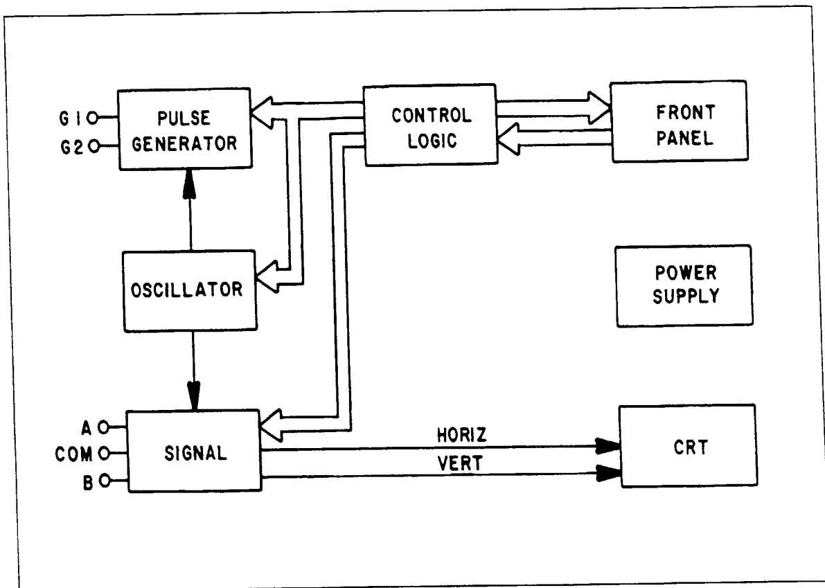
Figure 3-1. 2000 Block Diagram.
