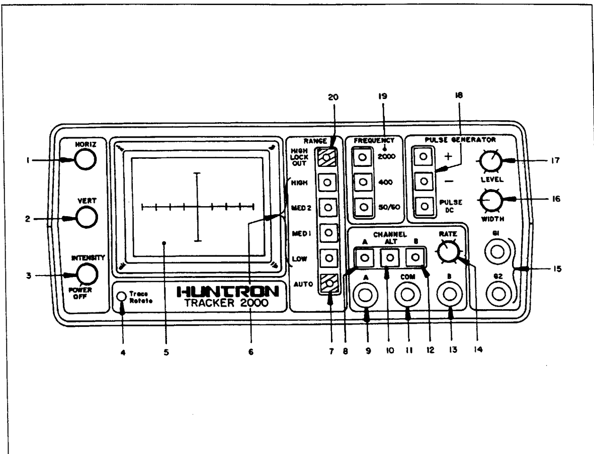
Figure 2-1. Front Panel.
