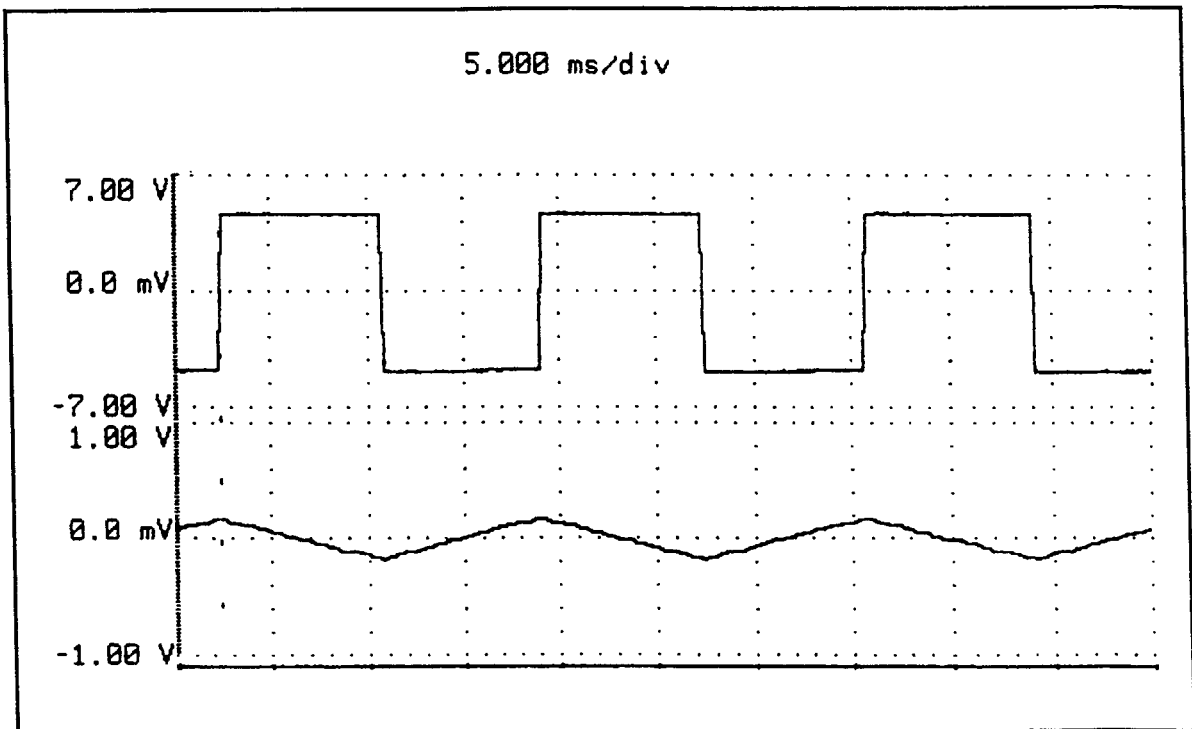
Figure 4-13. Signal PCB Waveforms: TP1 & TP6 - Settings: 50/60 Hz.
