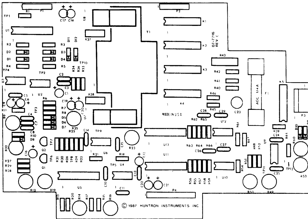
Figure 6-3. Signal PCB Component Locations
