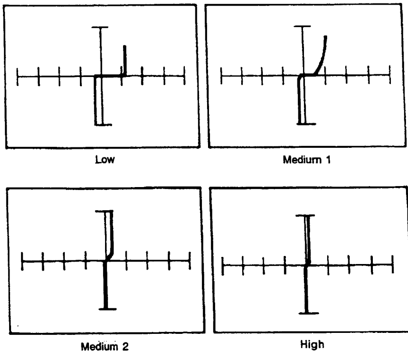
Figure 12-23. Signatures Between Pin 3 (Output) and Pin 1 of an LM555 Timer at 60 Hz.
