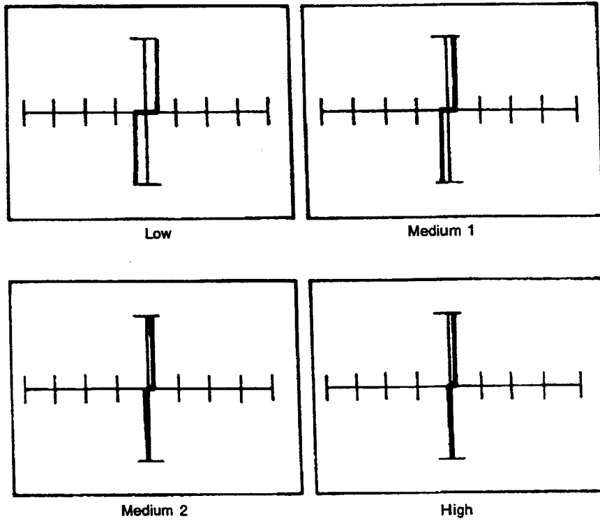
Figure 12-47. Signatures Between an Input Pin and V_{ss} - V_{dd} of a 4016B at 60 Hz.
