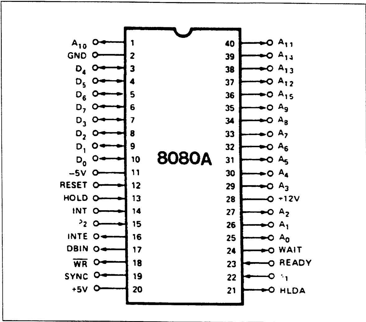
Figure 12-78. Pin Layout of an 8080A.
