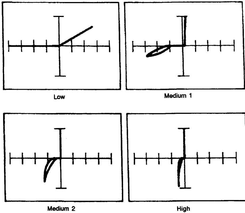
Figure 12-63. Signatures Between the V_{bb} Pin and the V_{SS} Pin of a 2708JL at 60 Hz.
