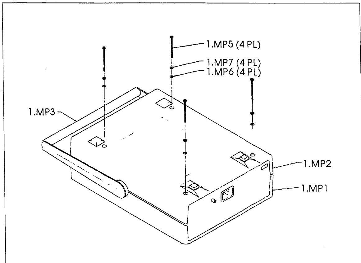
Figure 4-1. Case Screws Removal.
