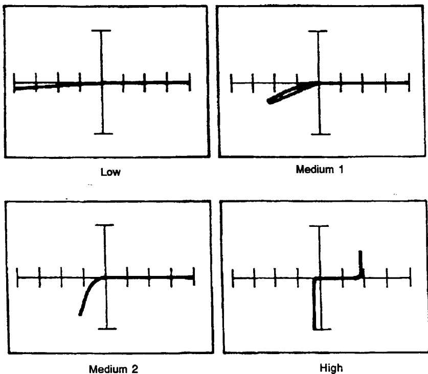
Figure 12-58. Signatures Between an Address Pin and the V_{ss} Pin of a 2708JL at 60 Hz.
