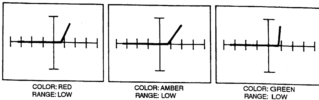
Figure 8-19. LED Signatures.
