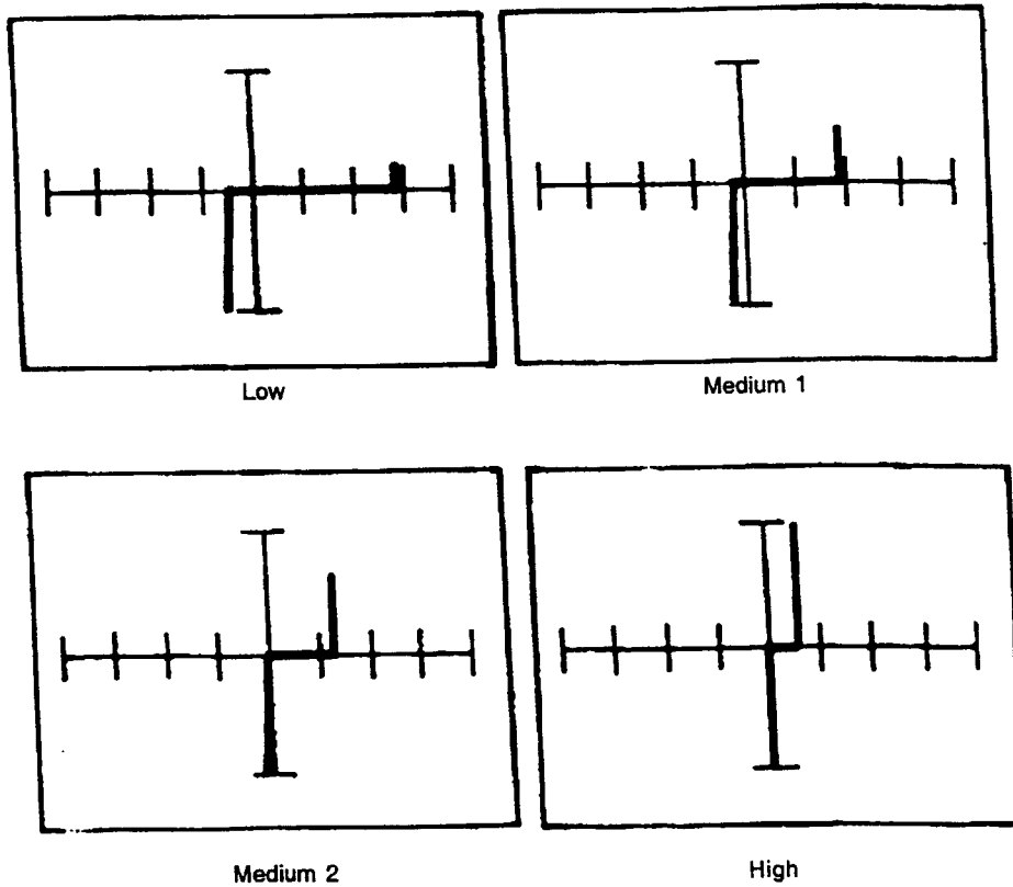
Figure 9-8. Signatures of a PNP Transistor (2N3906) at 60 Hz with Emitter as Common.
