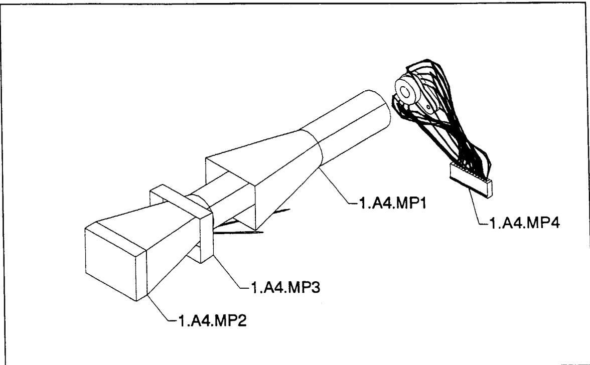
Figure 5-3. CRT Assembly.
