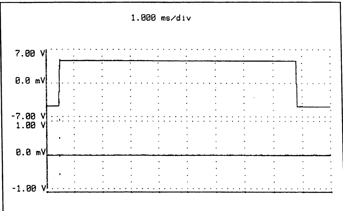
Figure 4-23. Signal PCB Waveforms: TP1 & TP12 - Settings: 2000 Hz, short circuit, LOW range.
