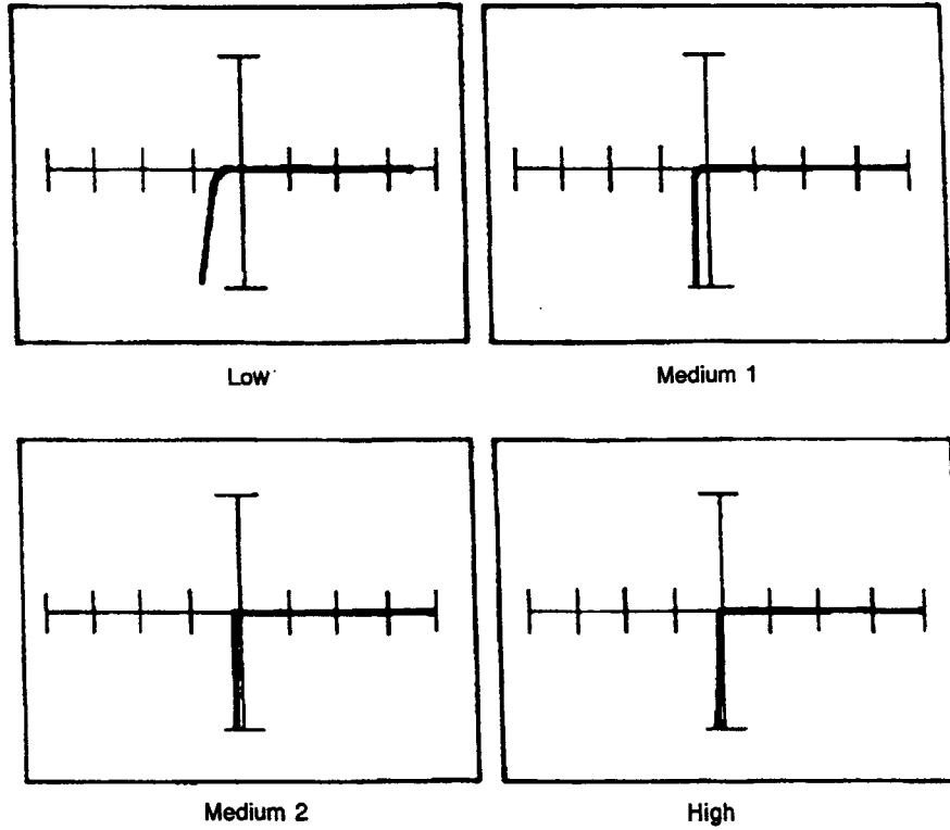
Figure 12-74. Signatures Between the V_{ref}(+) Pin and the V^- Pin of a DAC0800L at 60 Hz.
