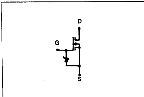
Figure 9-24. VN10KM MOSFET with a Gate-Source Protection Diode.
