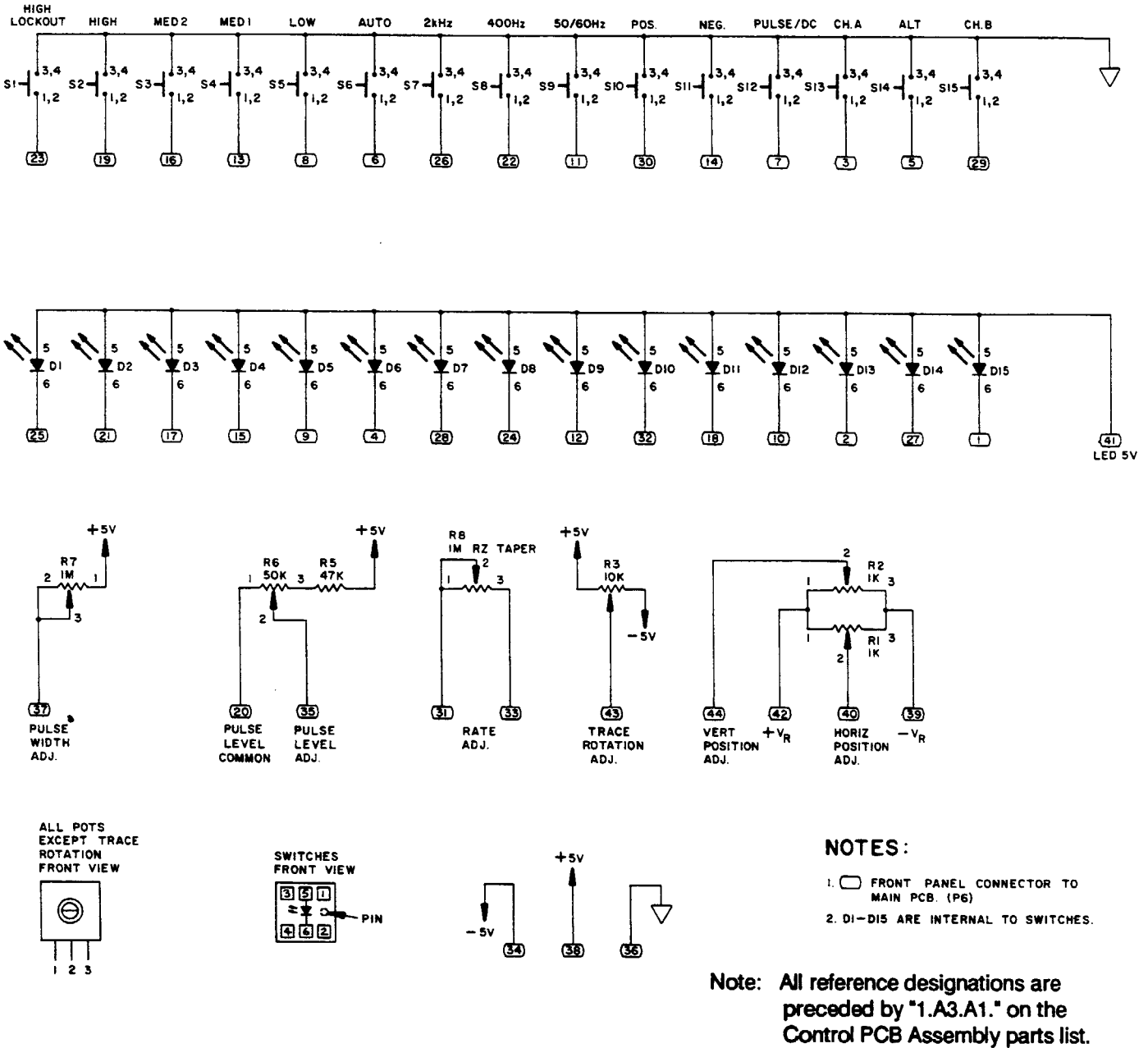
Figure 6-6. Control PCB Schematics
