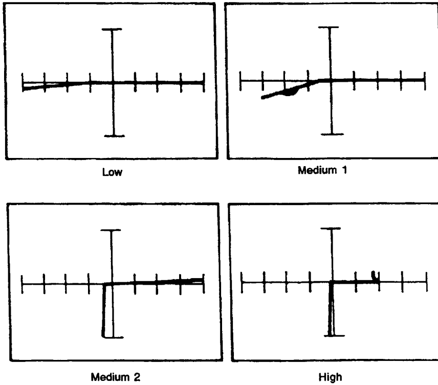
Figure 12-62. Signatures Between the CS Pin and the V_{SS} Pin of a 2708JL at 60 Hz.
