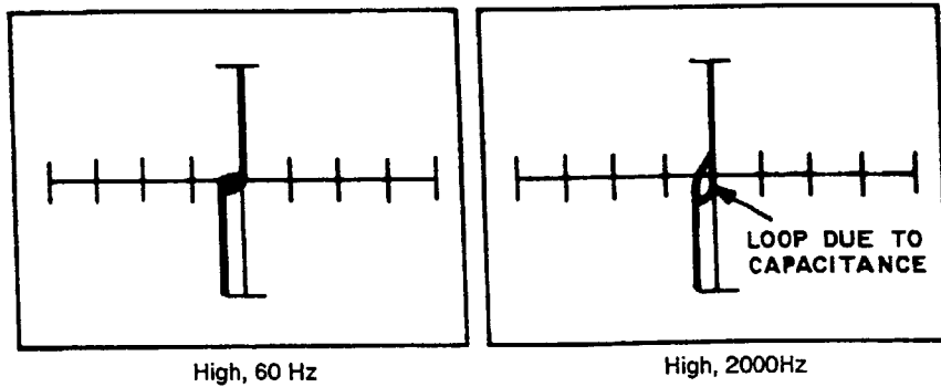
Figure 9-11. Signature of an NPN Power Transistor (TIP50) at 60 Hz and 2000 Hz. Base with Emitter as Common.
