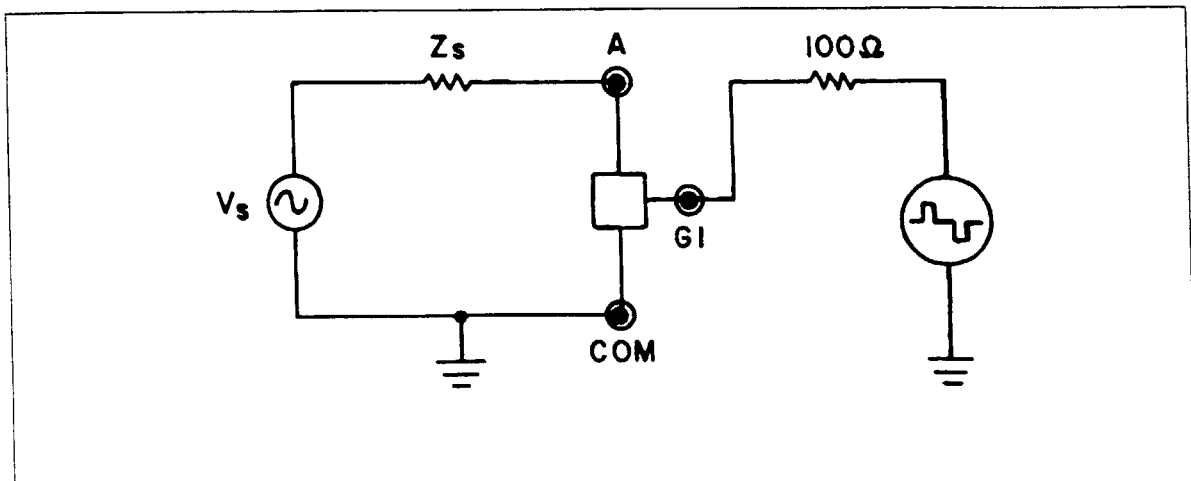
Figure 3-5. Pulse Generator/Signal Section Equivalent Circuit.
