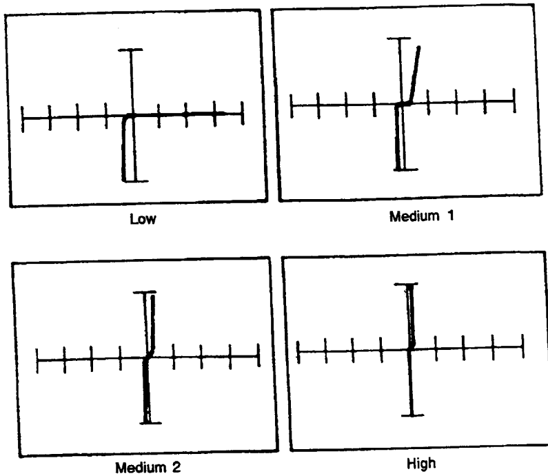
Figure 12-29. Signatures Between Pin 8 ( V_{cc} ) and Pin 1 of an LM555 Timer at 60 Hz.
