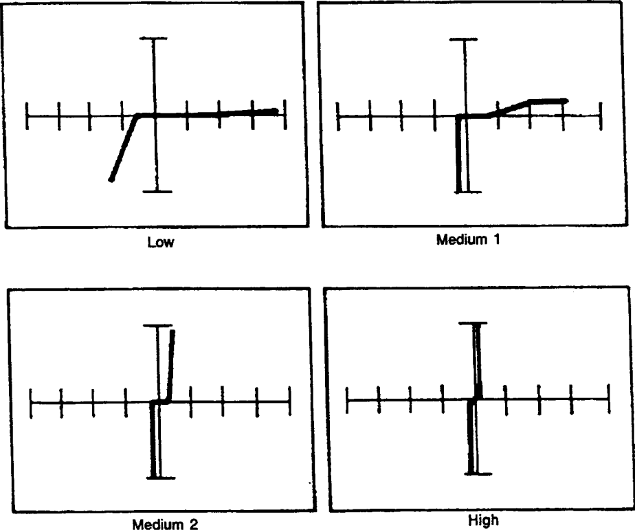
Figure 12-77. Signatures Between the V^+ and V^- Pins of a DAC0800L at 60 Hz.
