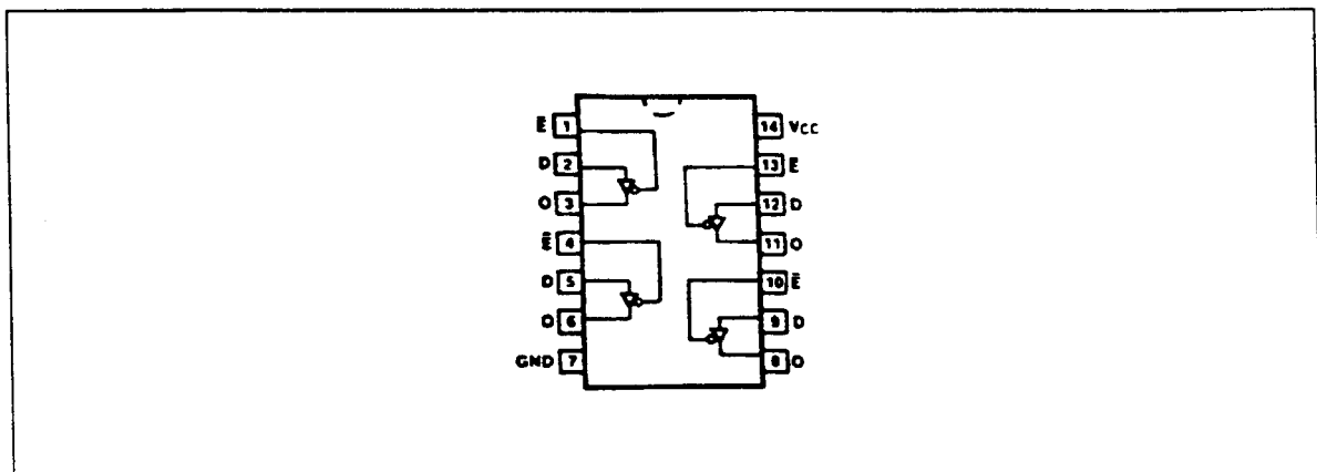
Figure 12-39. Pin Layout of a 74LS125.
