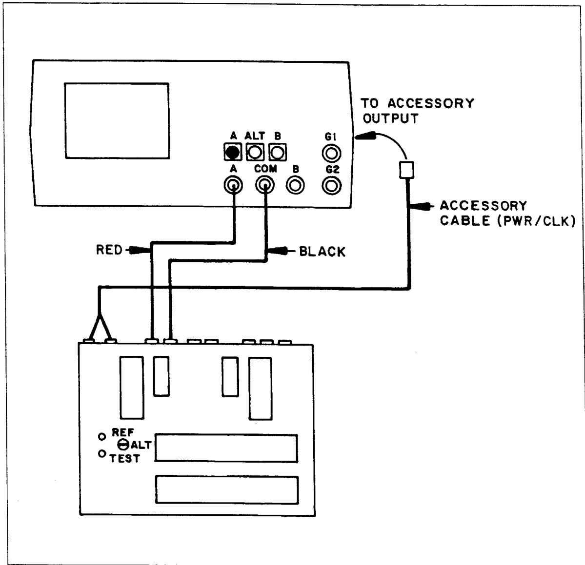
Figure 2-8. 2000/Switcher Interconnection.
