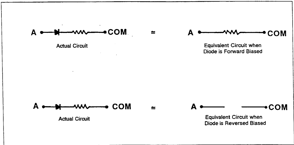
Figure 11-3. Diode/Resistor Equivalent Circuits.
