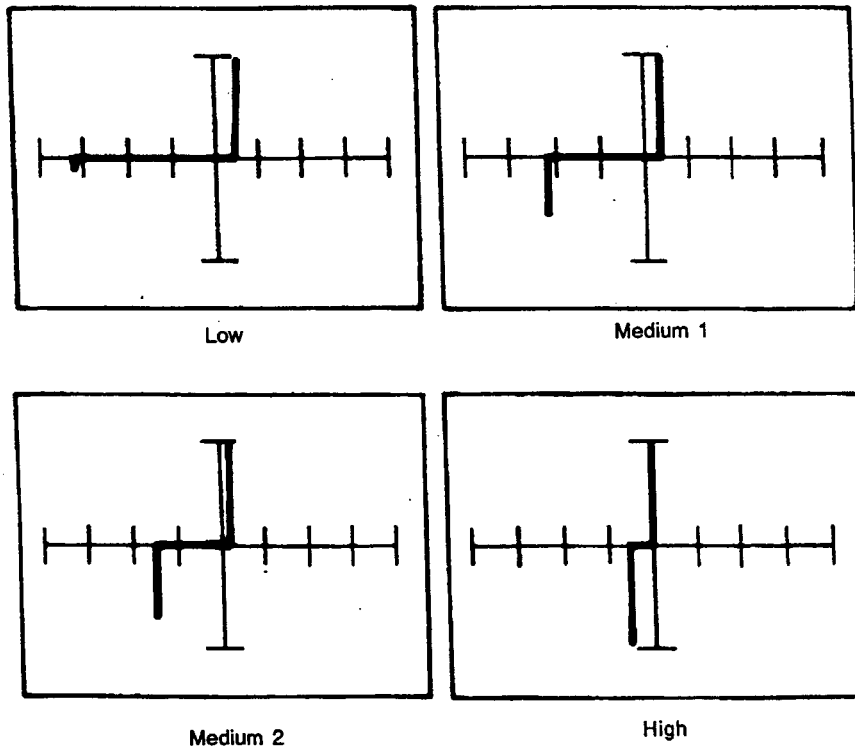
Figure 9-4. Signature of an NPN Transistor (2N3904) at 60 Hz Base with Emitter as Common.
