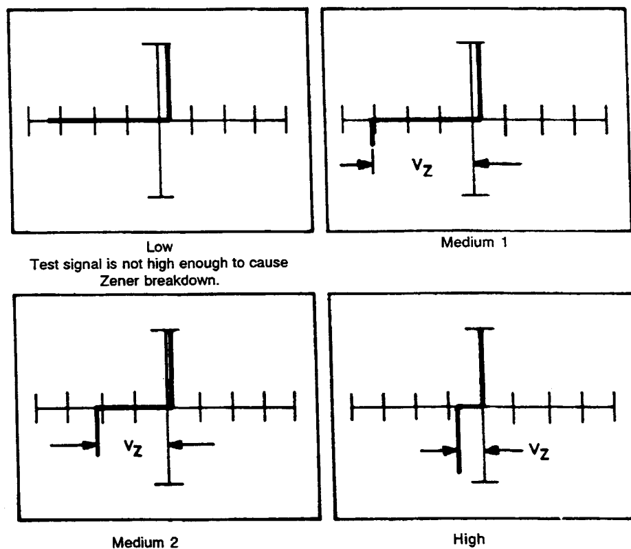
Figure 8-21. Signatures of a 1N5242 Zener Diode at 60 Hz.
