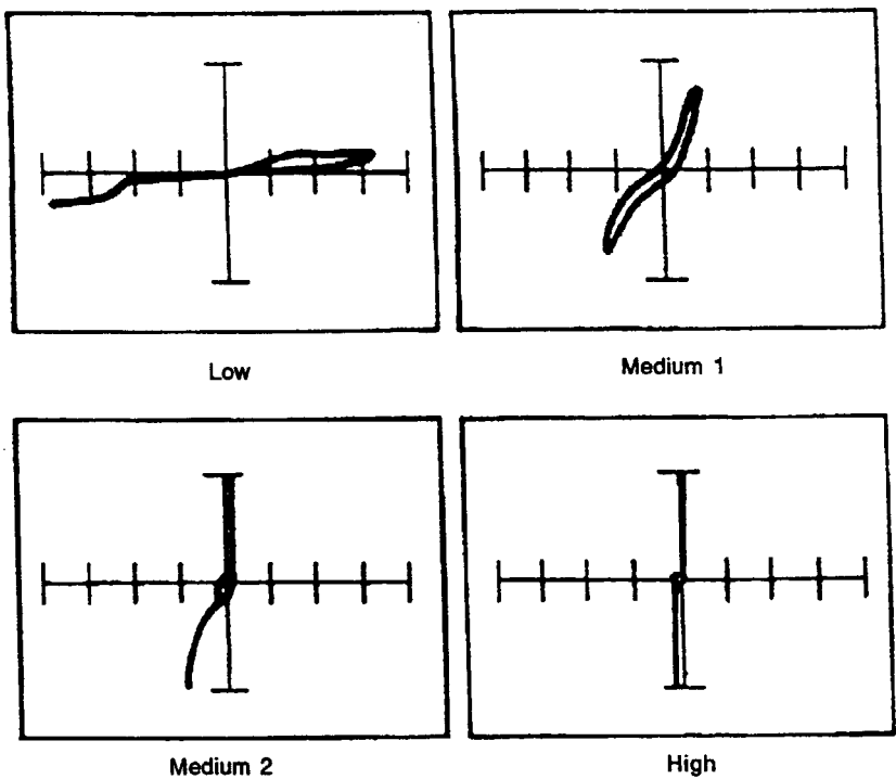
Figure 12-59. Signatures Between an Output Pin and the V_{ss} Pin of a 2708JL at 60 Hz.
