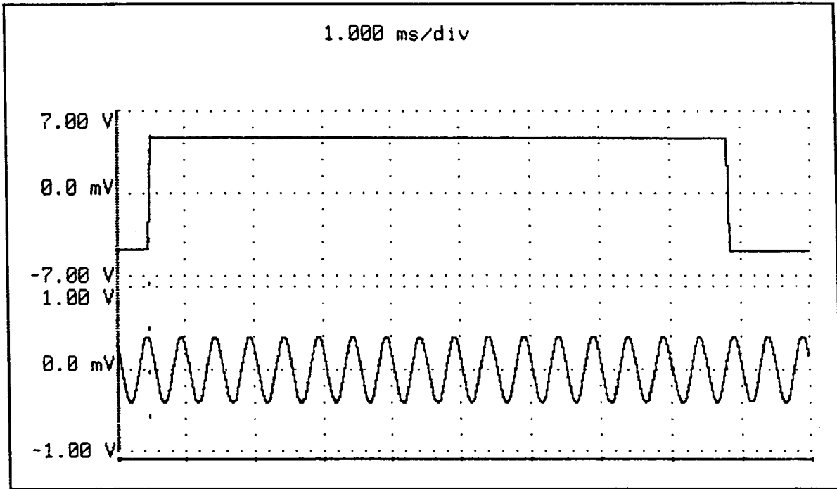
Figure 4-22. Signal PCB Waveforms: TP1 & TP12 - Settings: 2000 Hz, open circuit, LOW range.
