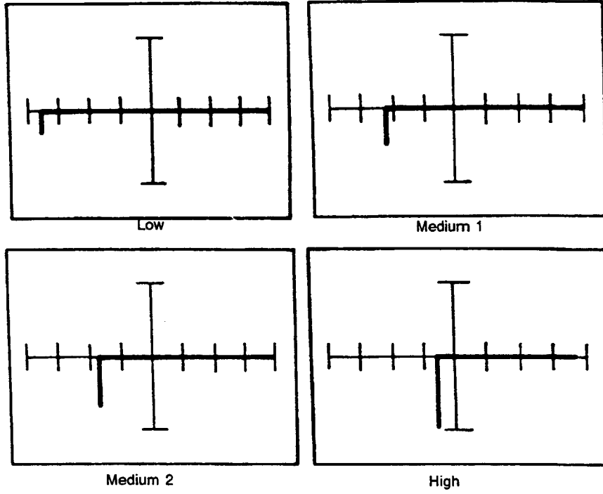
Figure 9-5. Signatures of an NPN Transistor (2N3904) at 60 Hz Collector with Base as Common.
