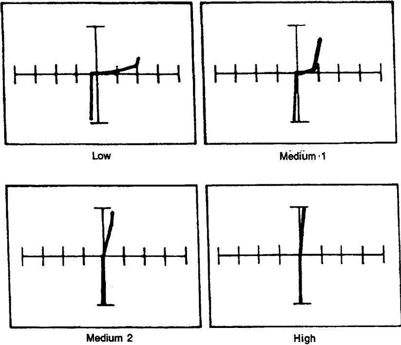
Figure 12-13. Signatures Between the Output and Ground Pins - 7805 at 60 Hz.
