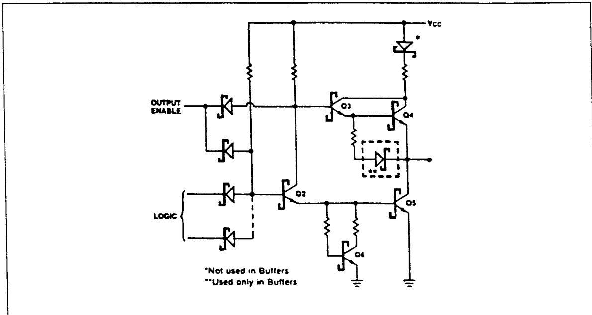
Figure 12-38. Typical Tri-State Output Control.
