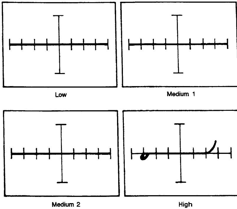
Figure 12-8. Signatures Between Pin 3 (Non-Inverting Input) and Pin 4 (V-) of an LM1458 at 60 Hz.
