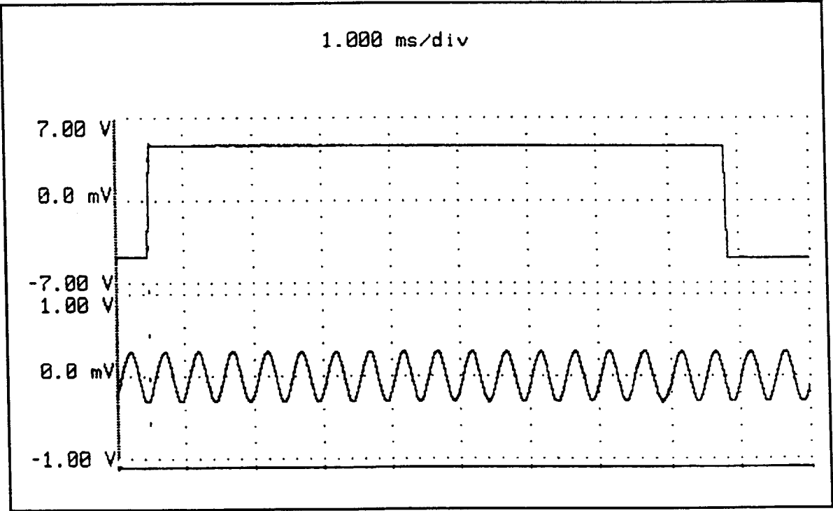
Figure 4-21. Signal PCB Waveforms: TP1 & TP11 - Settings: 2000 Hz, short circuit, LOW range.
