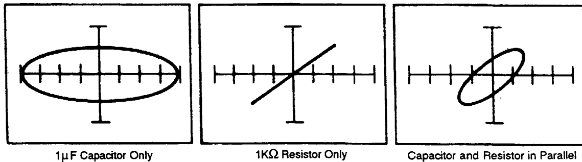
Figure 11-12. Effect of a 1\text{K}\Omega Resistor on a 1\mu\text{F} Capacitor in the Medium 1 Range at 60 Hz.
