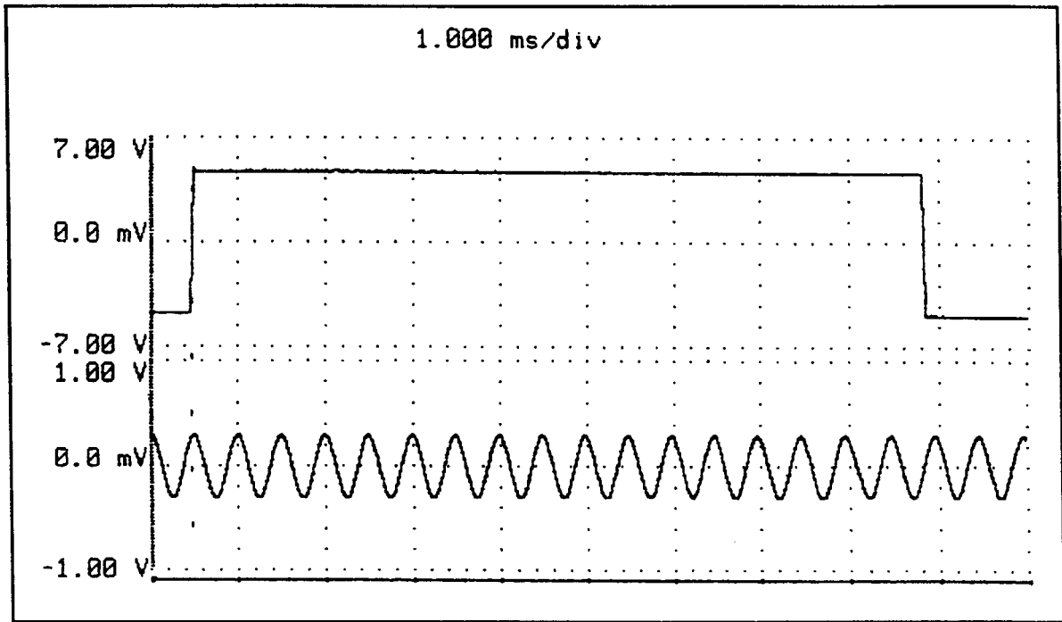
Figure 4-18. Signal PCB Waveforms: TP1 & TP9 - Settings: 2000 Hz.
