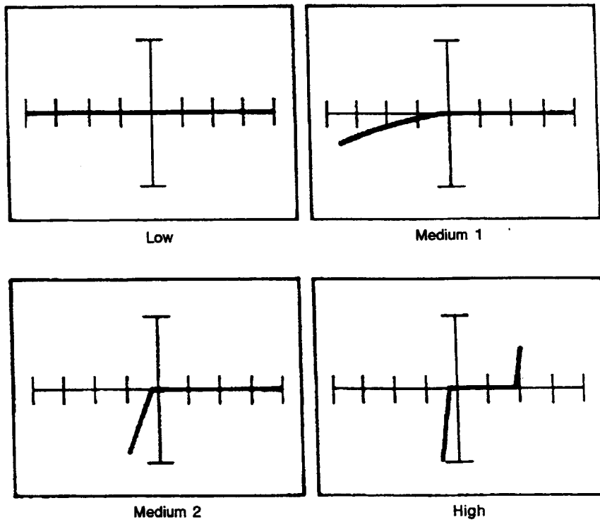
Figure 12-84. Signatures Between the INTE Pin and the -5V Pin of an 8080A at 60 Hz.
