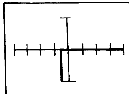
Figure 9-17. Signature Comparison of a Darlington Transistor (TIP112) and a Regular Transistor (TIP29) at 60 Hz. Collector with Emitter as Common.
