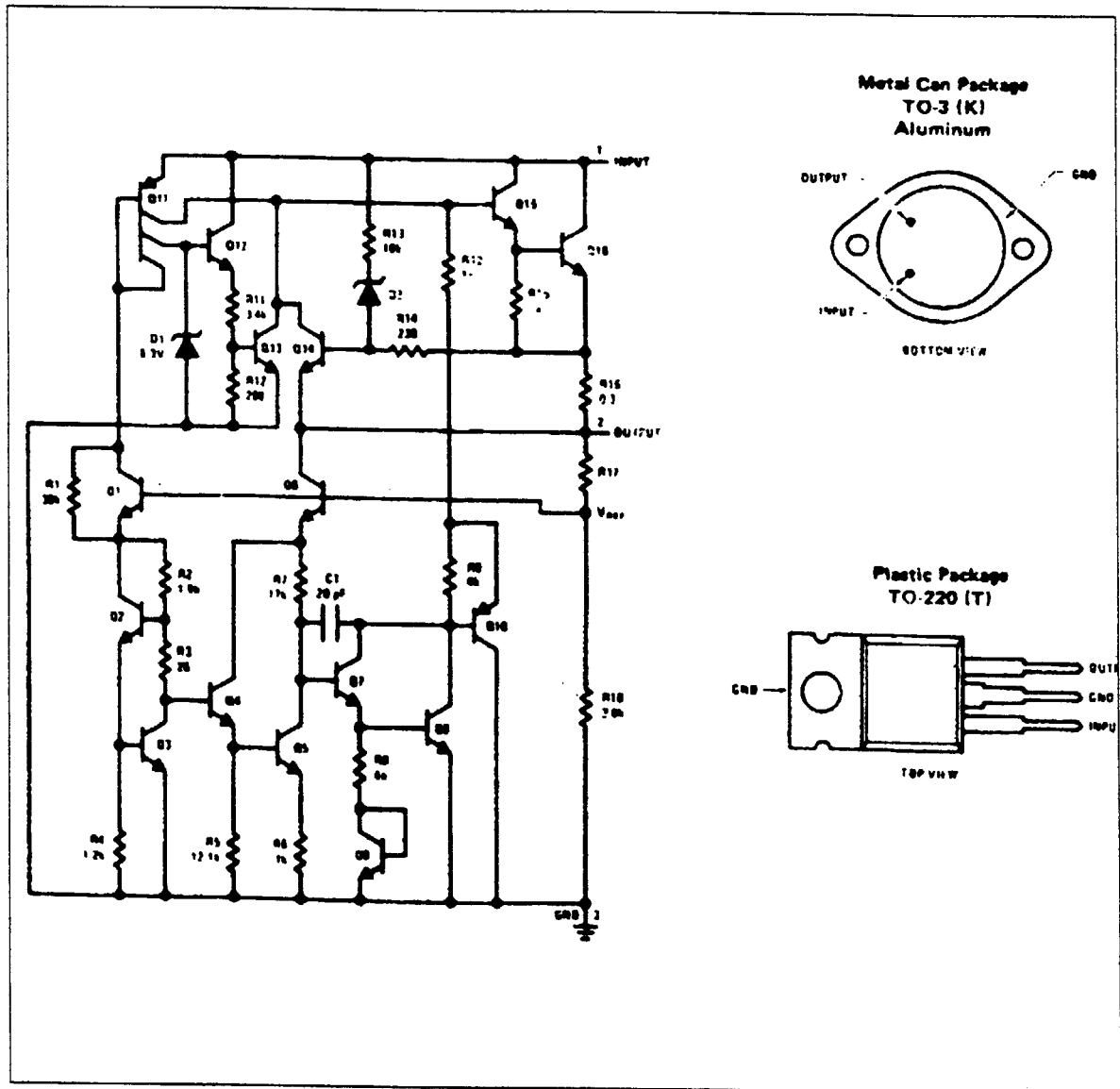
Figure 12-11. Schematic and Pin Layout of the 7805.
