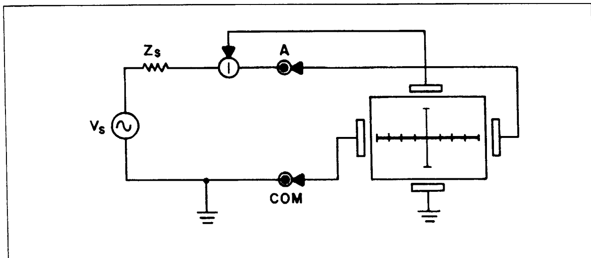
Figure 3-3. Signal Section Equivalent Circuit.
