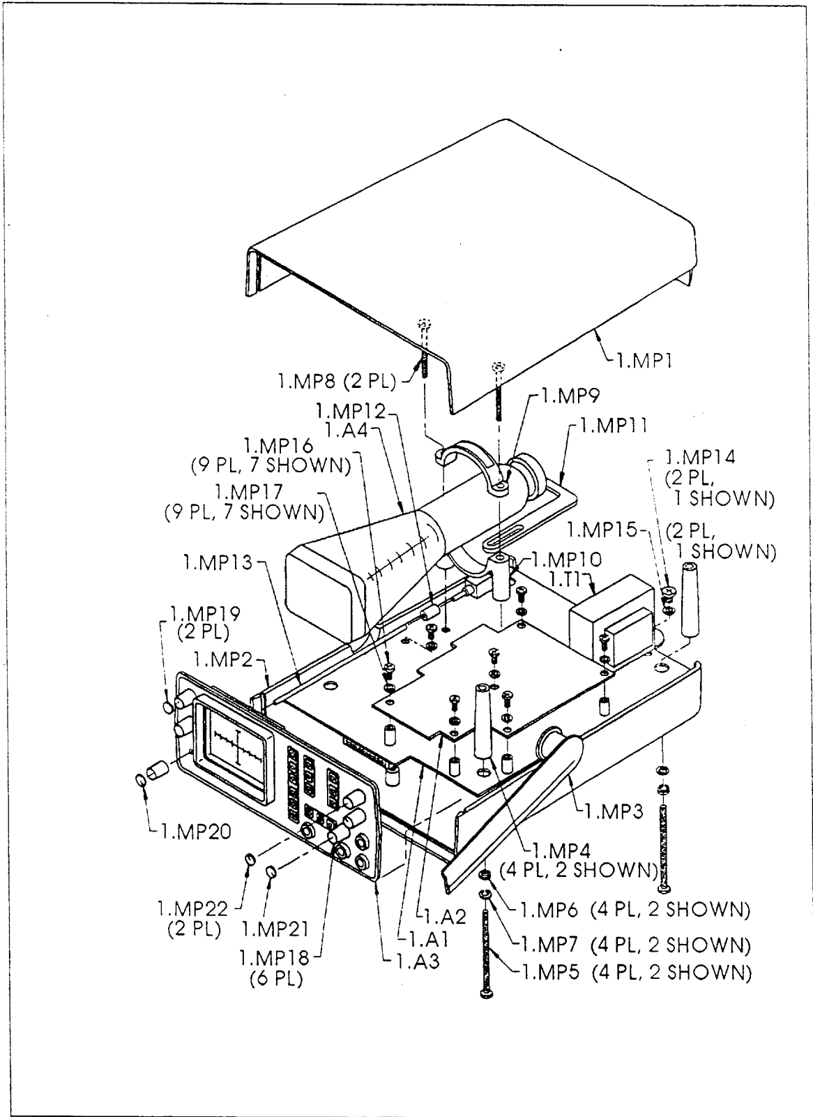
Figure 5-1. Final Assembly.
