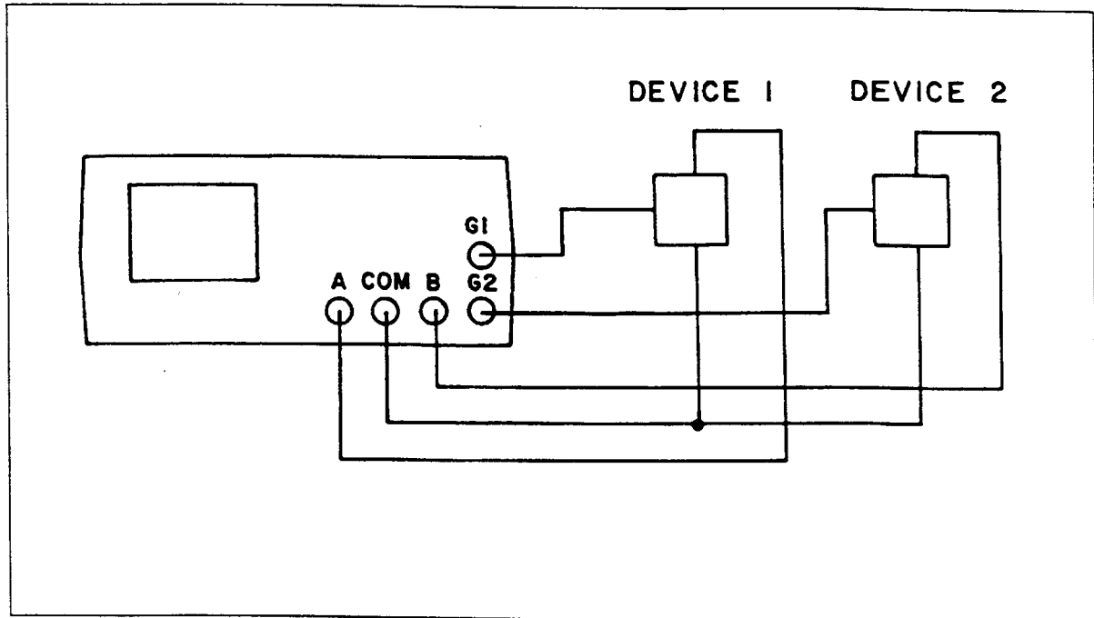
Figure 2-6. Pulse Generator Comparison Mode.
