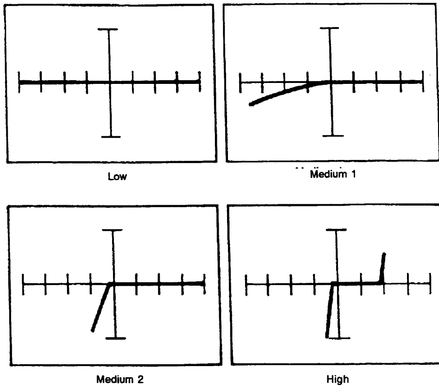
Figure 12-80. Signatures Between a Data Pin and the -5V Pin of an 8080A at 60 Hz.
