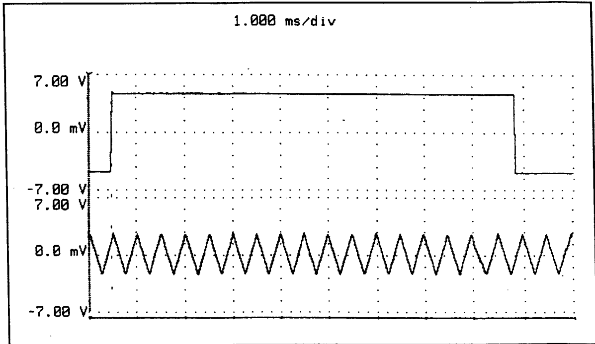
Figure 4-12. Signal PCB Waveforms: TP1 & TP5 - Settings: 2000 Hz.
