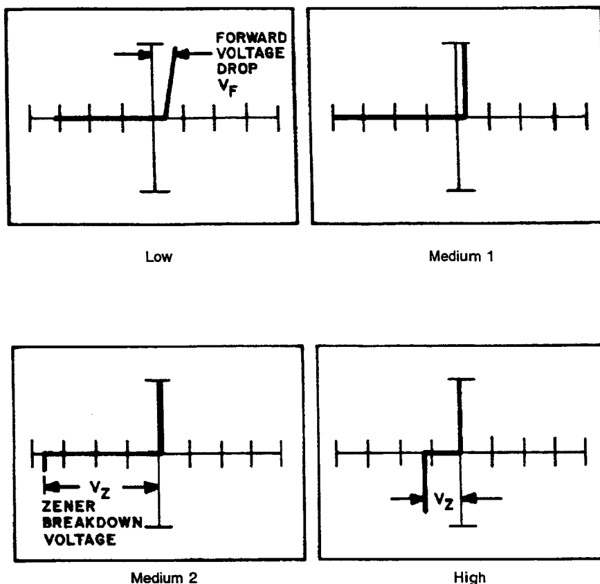
Figure 9-25. Signatures of an N-Channel Enhancement Mode MOSFET (VN10KM) at 60 Hz. Gate with Source as Common.
