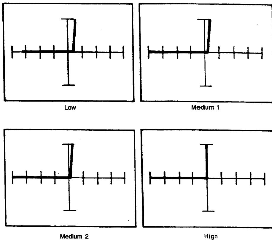
Figure 9-9. Signatures of a PNP Transistor (2N3906) at 60 Hz Collector with Base as Common.
