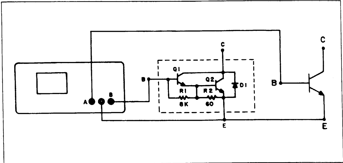
Figure 9-14. Base-Emitter Test Circuit.
