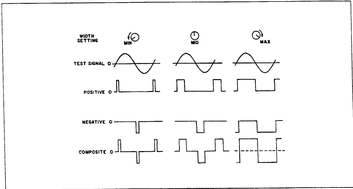
Figure 3-6. Pulse Generator Waveforms.
