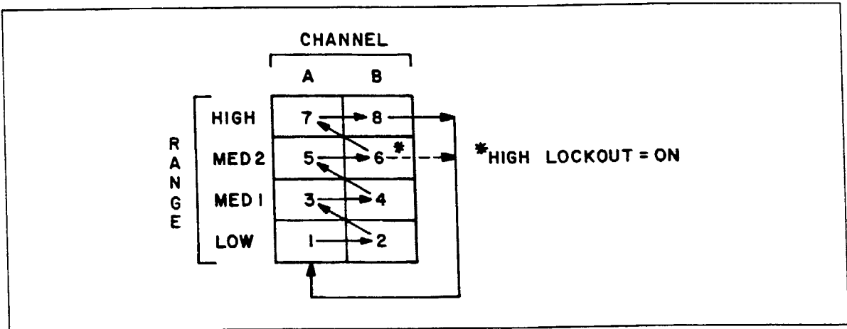
Figure 2-5. Auto/Alternate Sequence.
