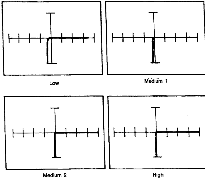
Figure 12-22. Signatures Between Pin 2 (Trigger) and Pin 1 of an LM555 Timer at 60 Hz.
