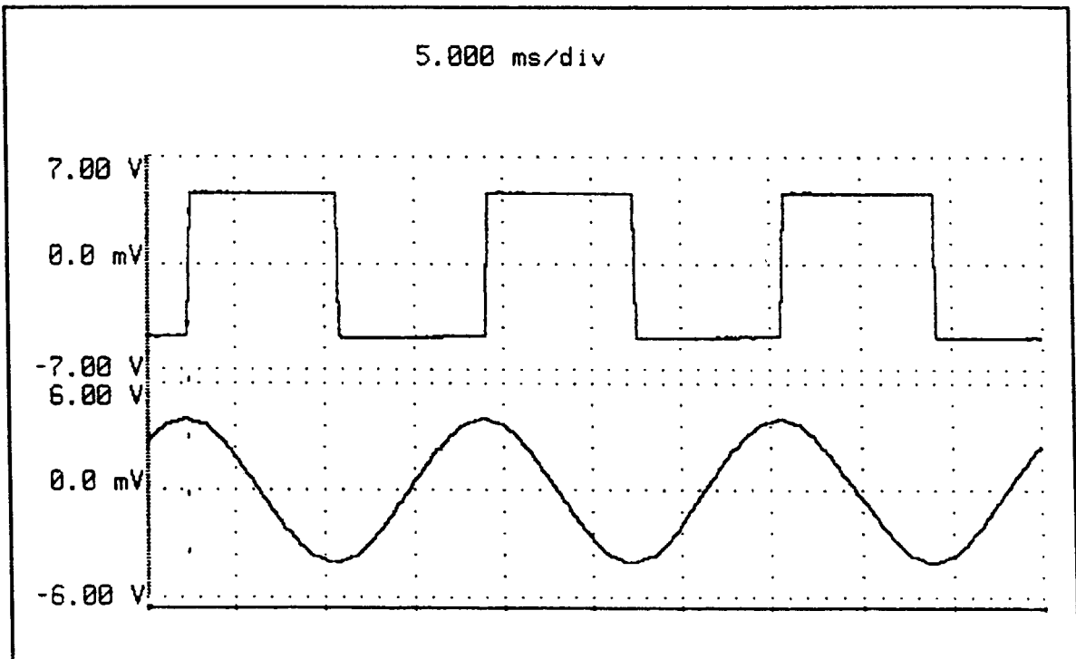
Figure 4-19. Signal PCB Waveforms: TP1 & TP10 - Settings: 50/60 Hz, LOW range.
